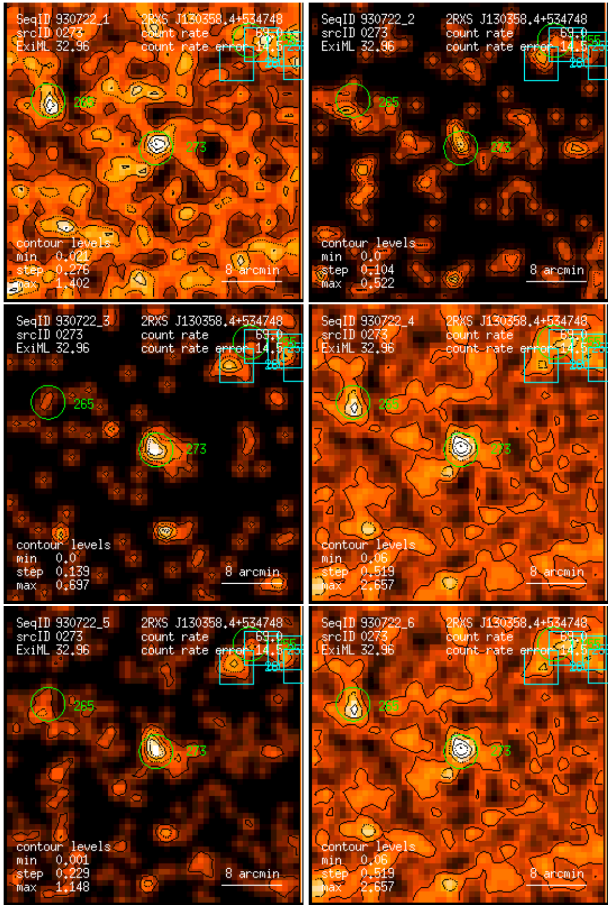
Figure 273: RASS 930722: detection 0273: band rate images, Gaussian filter: (1) PSPC channels 11 – 41, (2) 52 – 90, (3) 91 – 201, (4) 11 – 235, (5) 52 – 201, (6) 11 – 201. Broad band rates in counts/ks. Band rate contour levels in counts/ks/arcmin 2 .
