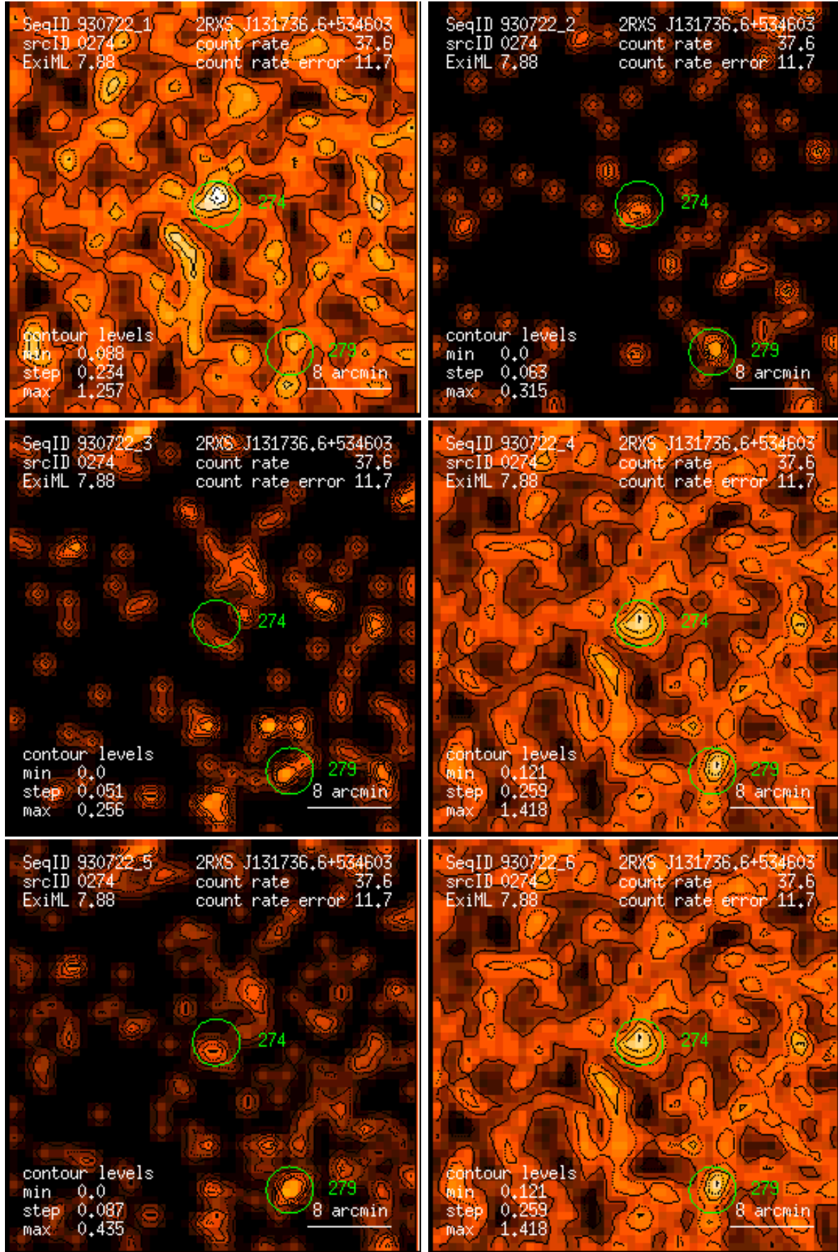
Figure 274: RASS 930722: detection 0274: band rate images, Gaussian filter: (1) PSPC channels 11 – 41, (2) 52 – 90, (3) 91 – 201, (4) 11 – 235, (5) 52 – 201, (6) 11 – 201. Broad band rates in counts/ks. Band rate contour levels in counts/ks/arcmin 2 .
