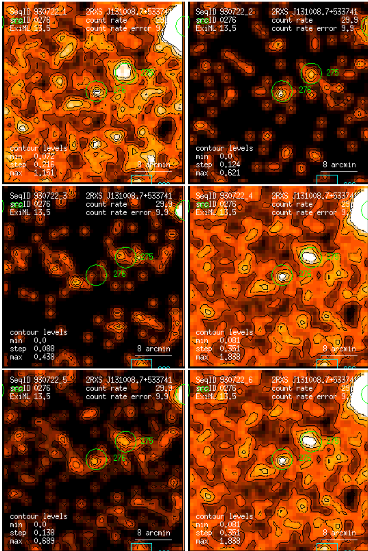
Figure 276: RASS 930722: detection 0276: band rate images, Gaussian filter: (1) PSPC channels 11 – 41, (2) 52 – 90, (3) 91 – 201, (4) 11 – 235, (5) 52 – 201, (6) 11 – 201. Broad band rates in counts/ks. Band rate contour levels in counts/ks/arcmin 2 .
