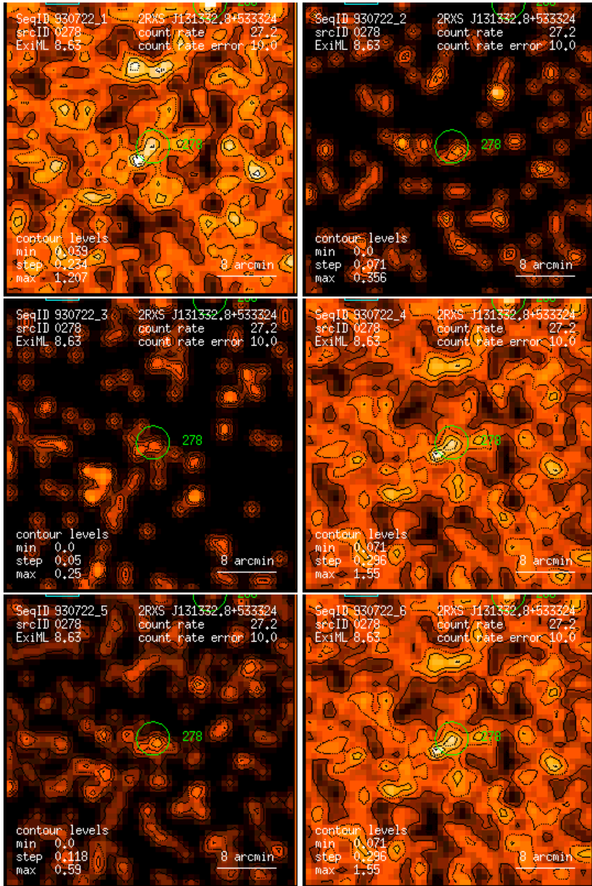
Figure 278: RASS 930722: detection 0278: band rate images, Gaussian filter: (1) PSPC channels 11 – 41, (2) 52 – 90, (3) 91 – 201, (4) 11 – 235, (5) 52 – 201, (6) 11 – 201. Broad band rates in counts/ks. Band rate contour levels in counts/ks/arcmin 2 .
