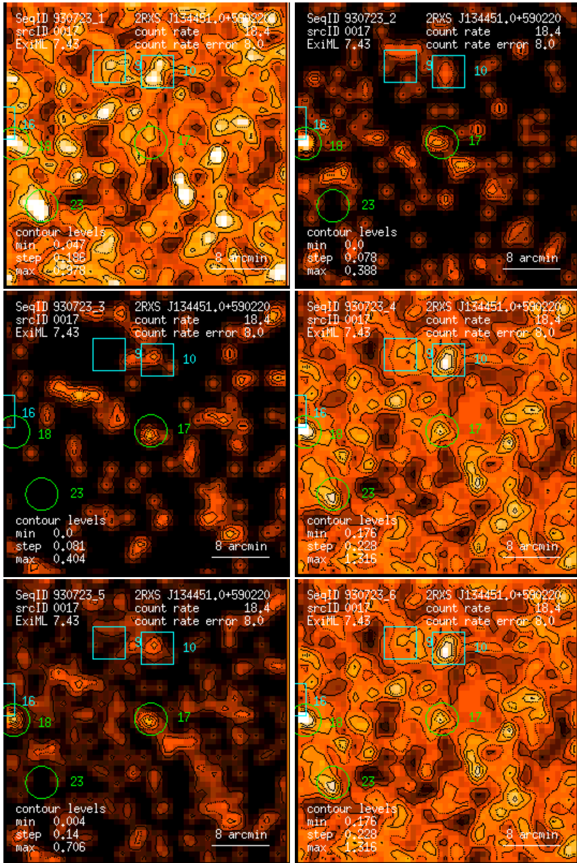
Figure 17: RASS 930723: detection 0017: band rate images, Gaussian filter: (1) PSPC channels 11 – 41, (2) 52 – 90, (3) 91 – 201, (4) 11 – 235, (5) 52 – 201, (6) 11 – 201. Broad band rates in counts/ks. Band rate contour levels in counts/ks/arcmin 2 .
