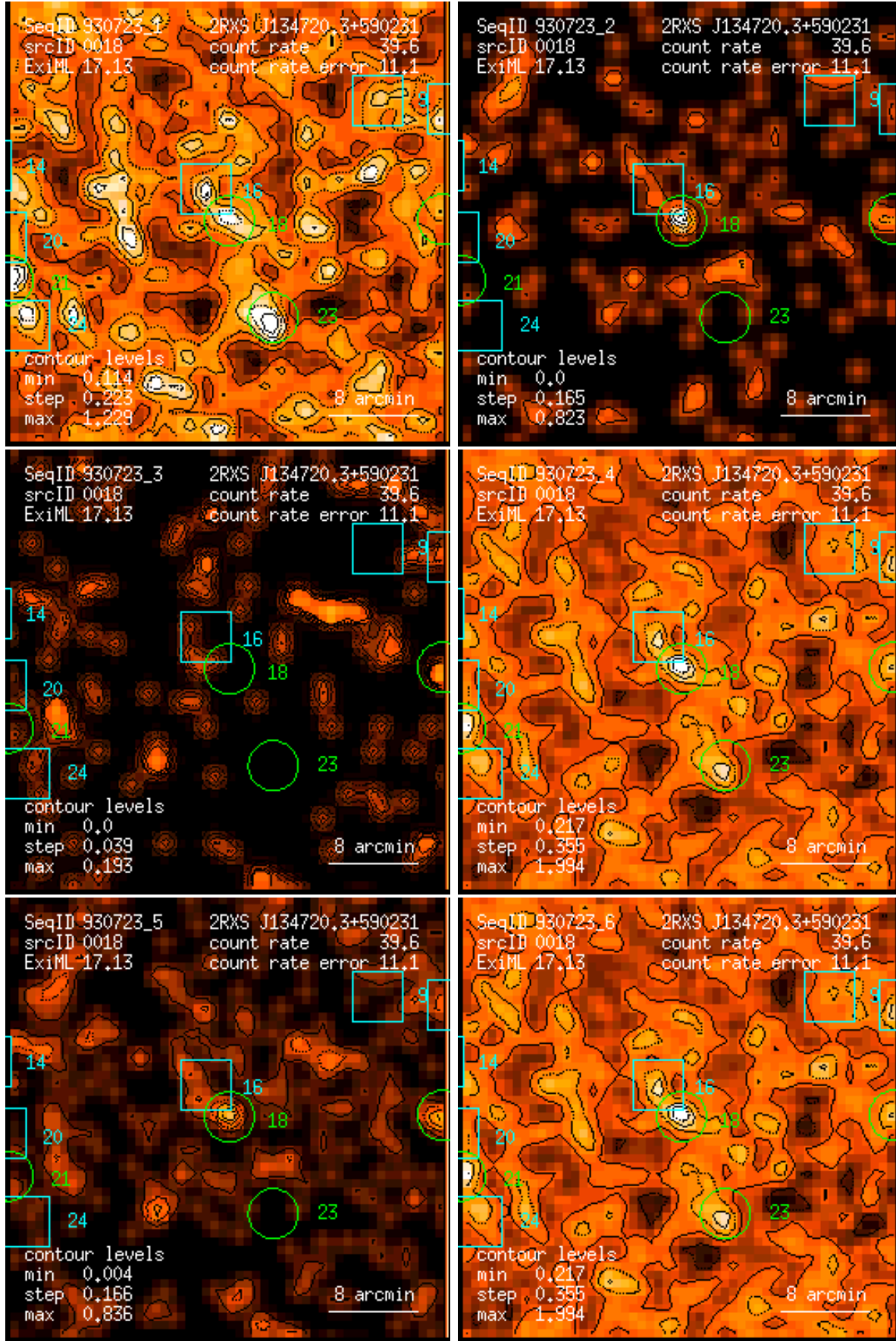
Figure 18: RASS 930723: detection 0018: band rate images, Gaussian filter: (1) PSPC channels 11 – 41, (2) 52 – 90, (3) 91 – 201, (4) 11 – 235, (5) 52 – 201, (6) 11 – 201. Broad band rates in counts/ks. Band rate contour levels in counts/ks/arcmin 2 .
