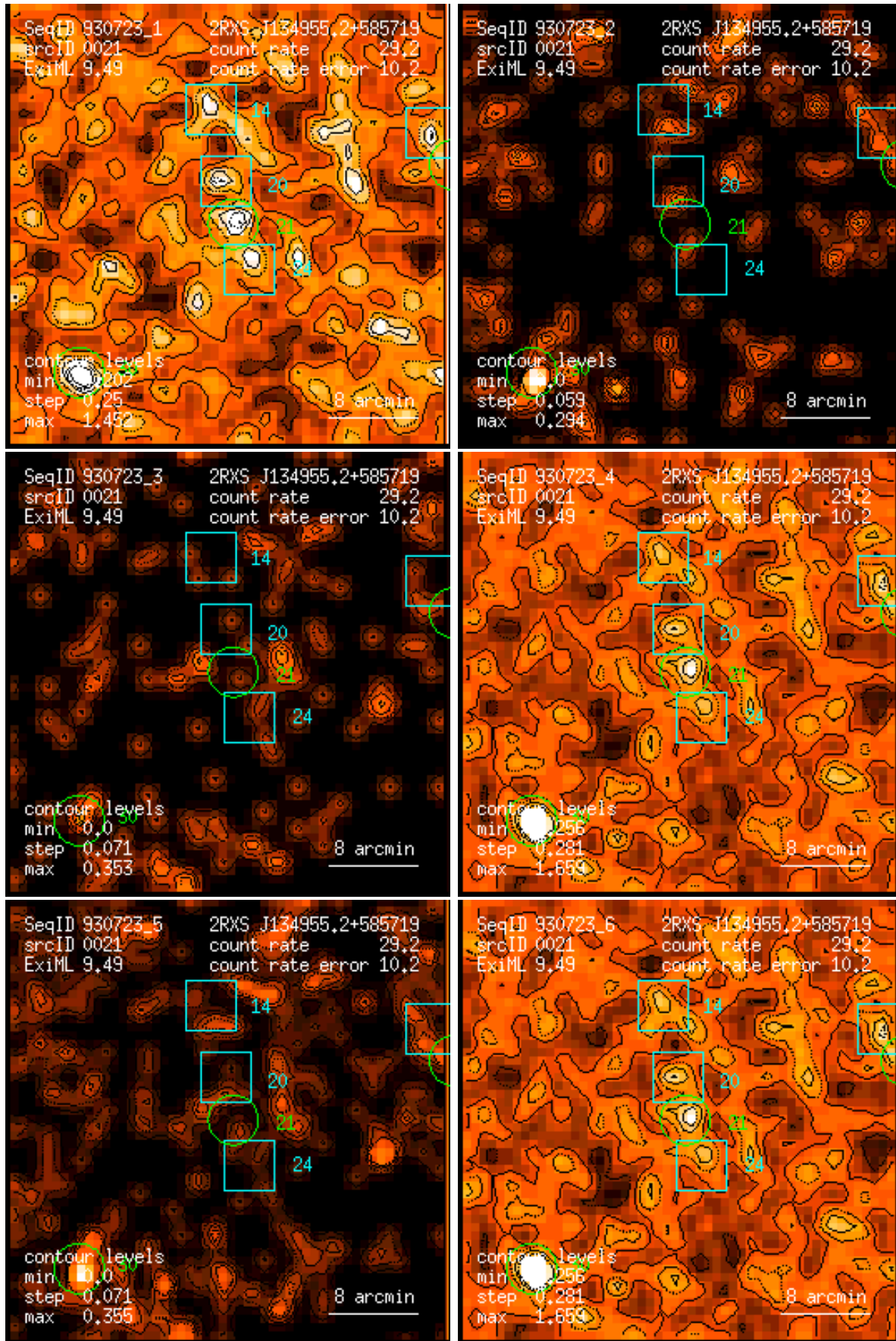
Figure 21: RASS 930723: detection 0021: band rate images, Gaussian filter: (1) PSPC channels 11 – 41, (2) 52 – 90, (3) 91 – 201, (4) 11 – 235, (5) 52 – 201, (6) 11 – 201. Broad band rates in counts/ks. Band rate contour levels in counts/ks/arcmin 2 .
