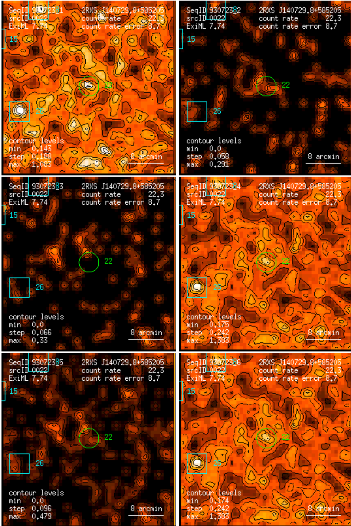
Figure 22: RASS 930723: detection 0022: band rate images, Gaussian filter: (1) PSPC channels 11 – 41, (2) 52 – 90, (3) 91 – 201, (4) 11 – 235, (5) 52 – 201, (6) 11 – 201. Broad band rates in counts/ks. Band rate contour levels in counts/ks/arcmin 2 .
