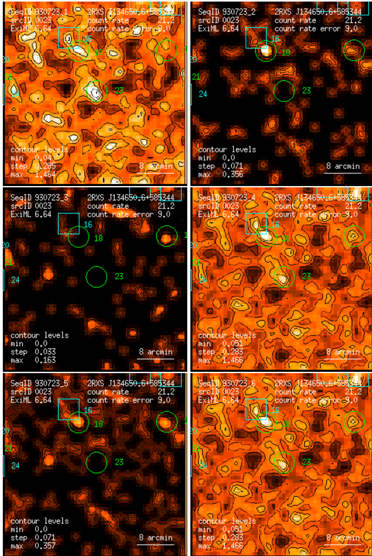
Figure 23: RASS 930723: detection 0023: band rate images, Gaussian filter: (1) PSPC channels 11 – 41, (2) 52 – 90, (3) 91 – 201, (4) 11 – 235, (5) 52 – 201, (6) 11 – 201. Broad band rates in counts/ks. Band rate contour levels in counts/ks/arcmin 2 .
