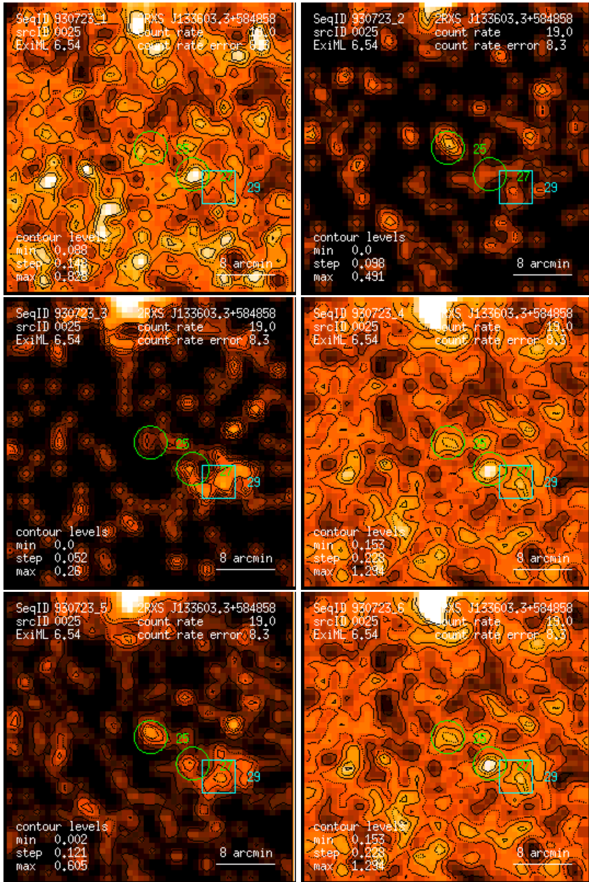
Figure 25: RASS 930723: detection 0025: band rate images, Gaussian filter: (1) PSPC channels 11 – 41, (2) 52 – 90, (3) 91 – 201, (4) 11 – 235, (5) 52 – 201, (6) 11 – 201. Broad band rates in counts/ks. Band rate contour levels in counts/ks/arcmin 2 .
