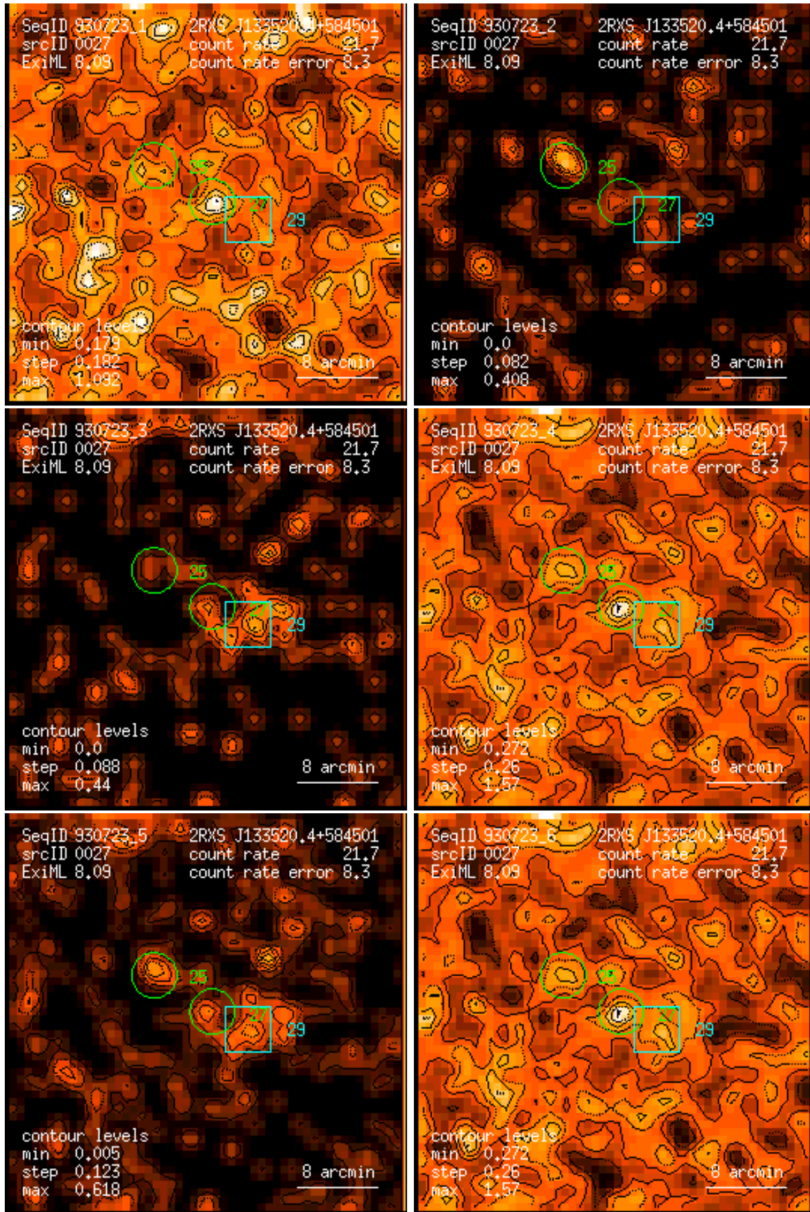
Figure 27: RASS 930723: detection 0027: band rate images, Gaussian filter: (1) PSPC channels 11 – 41, (2) 52 – 90, (3) 91 – 201, (4) 11 – 235, (5) 52 – 201, (6) 11 – 201. Broad band rates in counts/ks. Band rate contour levels in counts/ks/arcmin 2 .
