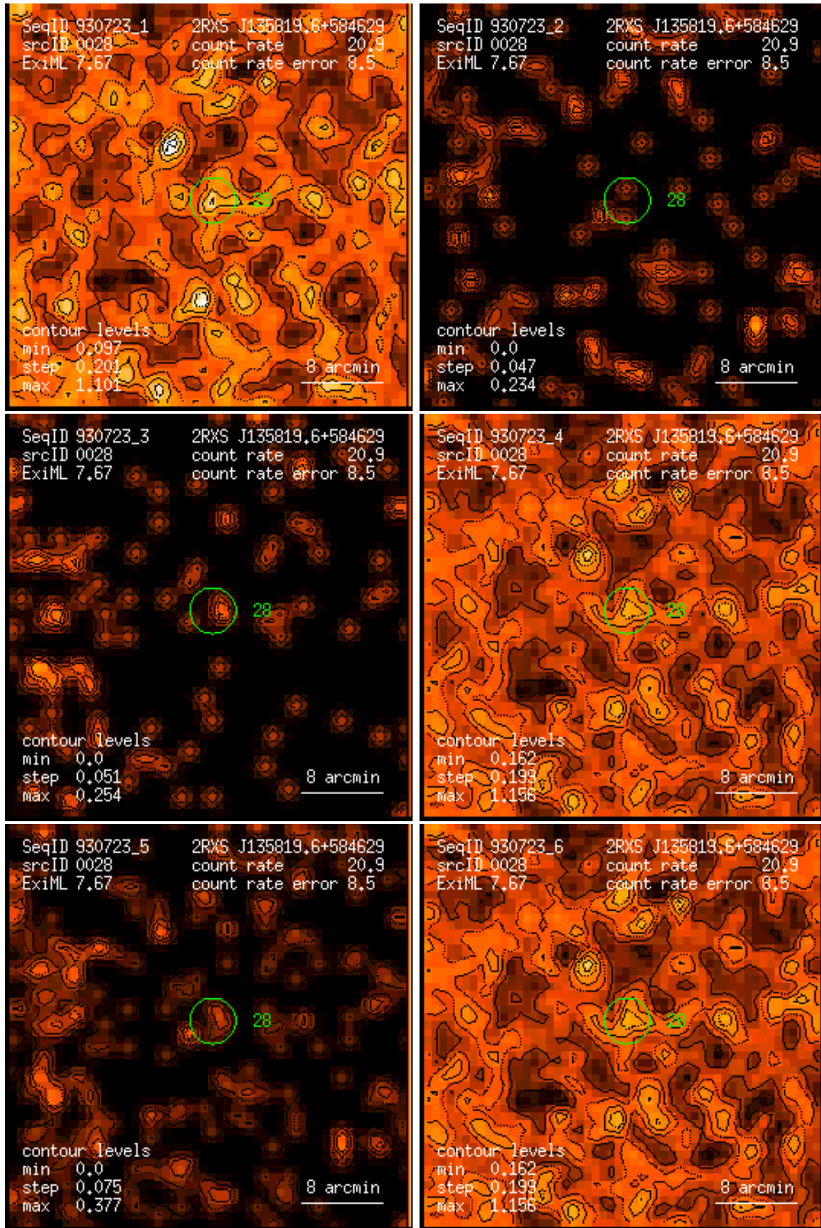
Figure 28: RASS 930723: detection 0028: band rate images, Gaussian filter: (1) PSPC channels 11 – 41, (2) 52 – 90, (3) 91 – 201, (4) 11 – 235, (5) 52 – 201, (6) 11 – 201. Broad band rates in counts/ks. Band rate contour levels in counts/ks/arcmin 2 .
