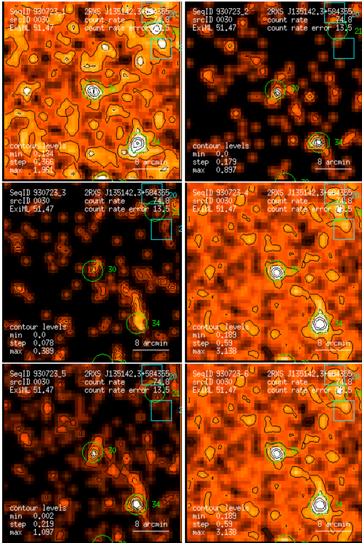
Figure 30: RASS 930723: detection 0030: band rate images, Gaussian filter: (1) PSPC channels 11 – 41, (2) 52 – 90, (3) 91 – 201, (4) 11 – 235, (5) 52 – 201, (6) 11 – 201. Broad band rates in counts/ks. Band rate contour levels in counts/ks/arcmin 2 .
