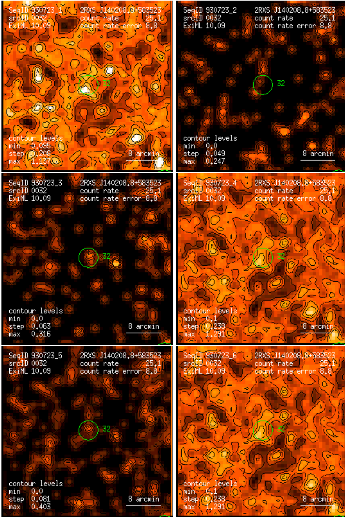
Figure 32: RASS 930723: detection 0032: band rate images, Gaussian filter: (1) PSPC channels 11 – 41, (2) 52 – 90, (3) 91 – 201, (4) 11 – 235, (5) 52 – 201, (6) 11 – 201. Broad band rates in counts/ks. Band rate contour levels in counts/ks/arcmin 2 .
