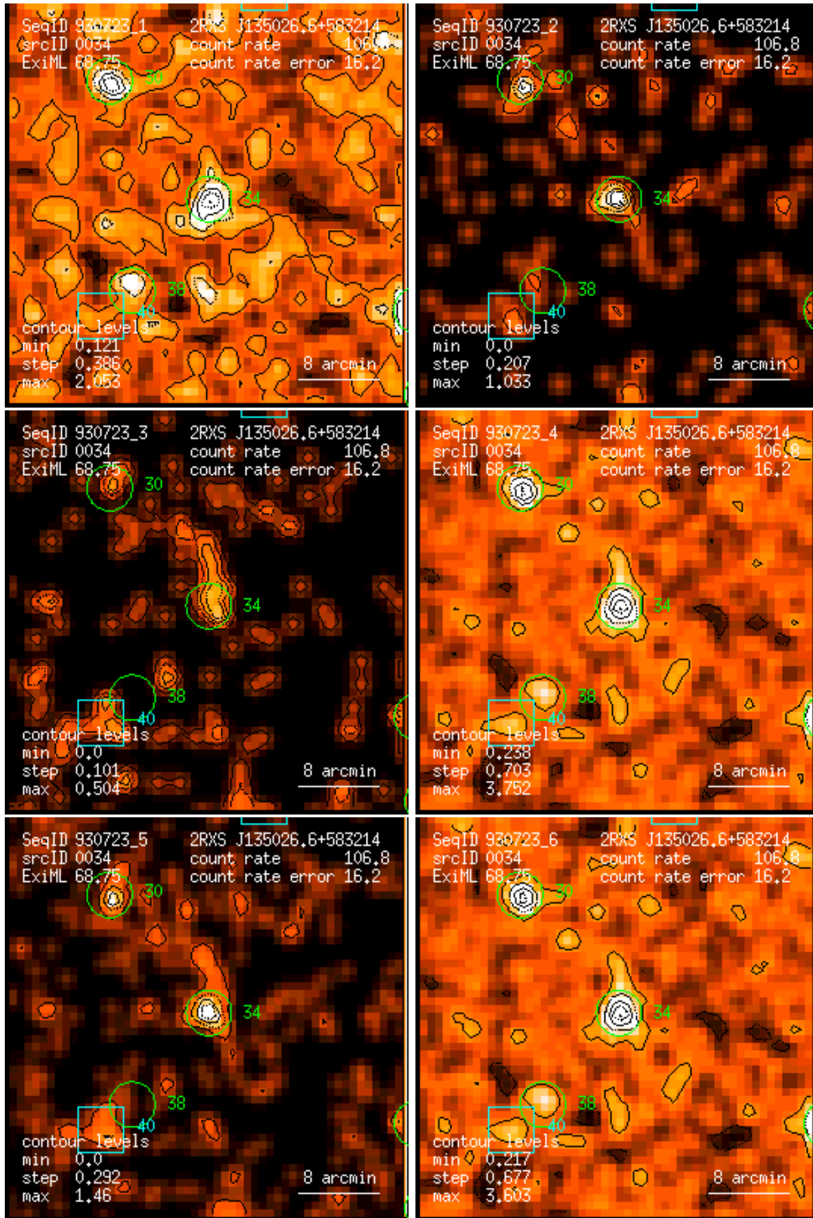
Figure 34: RASS 930723: detection 0034: band rate images, Gaussian filter: (1) PSPC channels 11 – 41, (2) 52 – 90, (3) 91 – 201, (4) 11 – 235, (5) 52 – 201, (6) 11 – 201. Broad band rates in counts/ks. Band rate contour levels in counts/ks/arcmin 2 .
