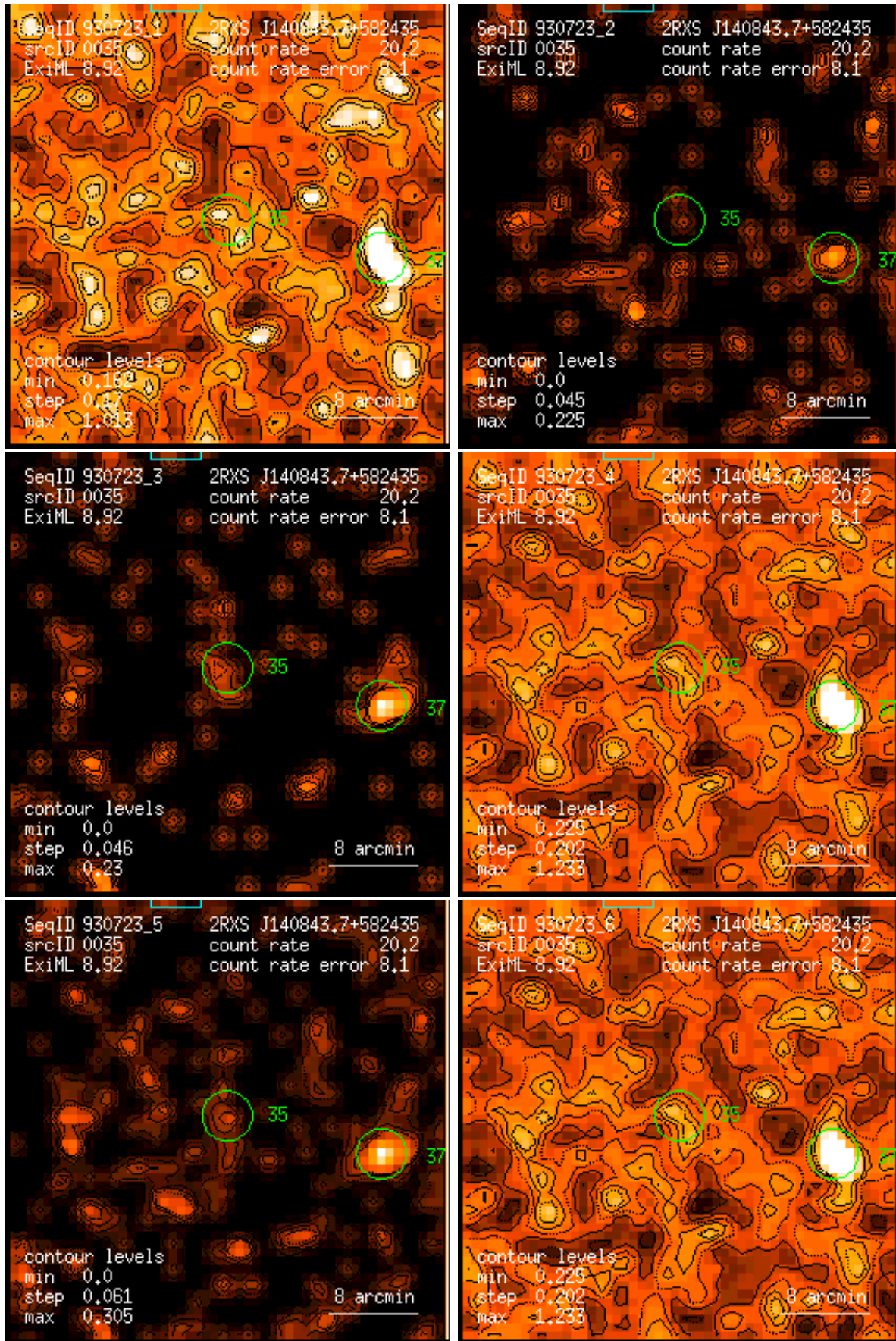
Figure 35: RASS 930723: detection 0035: band rate images, Gaussian filter: (1) PSPC channels 11 – 41, (2) 52 – 90, (3) 91 – 201, (4) 11 – 235, (5) 52 – 201, (6) 11 – 201. Broad band rates in counts/ks. Band rate contour levels in counts/ks/arcmin 2 .
