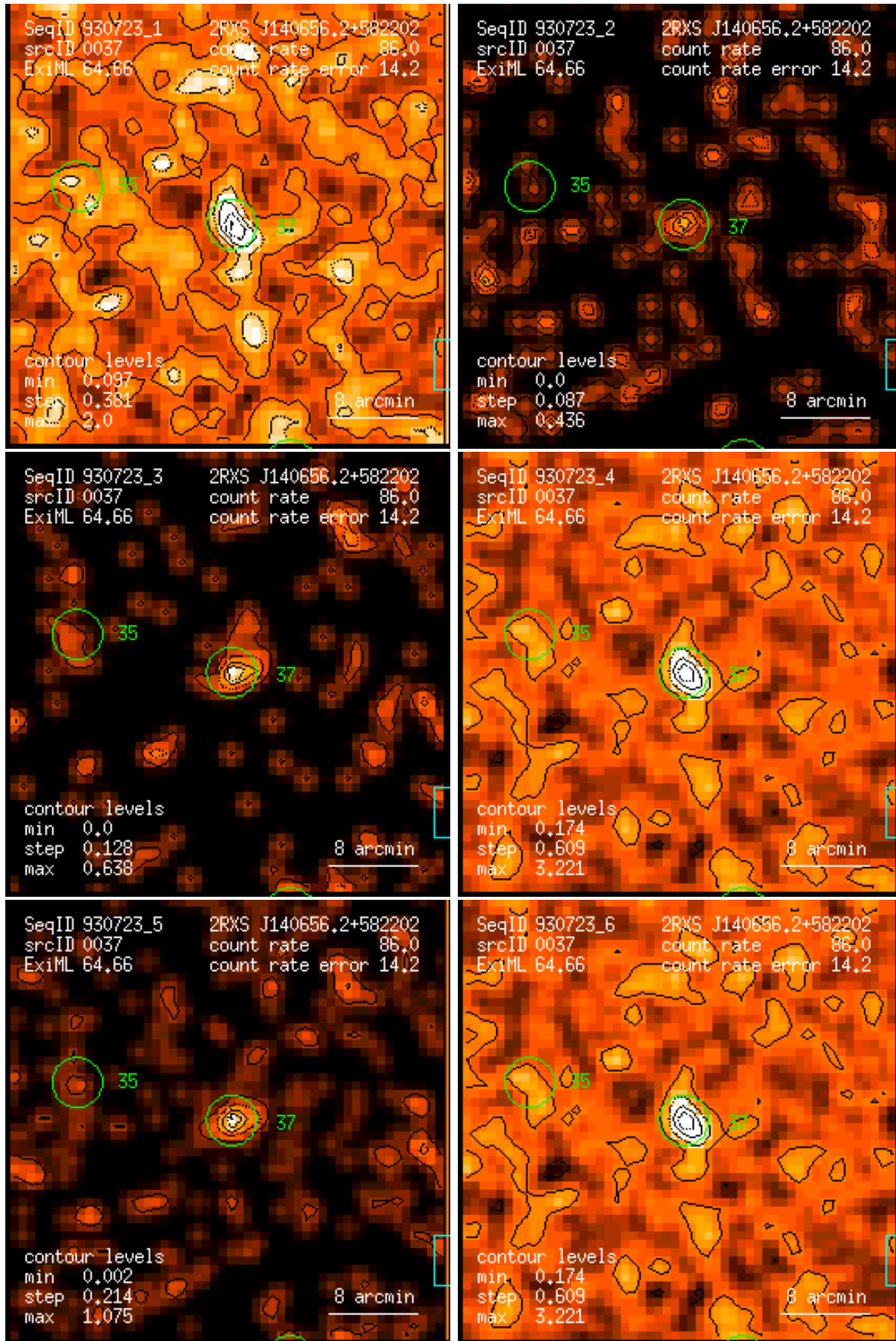
Figure 37: RASS 930723: detection 0037: band rate images, Gaussian filter: (1) PSPC channels 11 – 41, (2) 52 – 90, (3) 91 – 201, (4) 11 – 235, (5) 52 – 201, (6) 11 – 201. Broad band rates in counts/ks. Band rate contour levels in counts/ks/arcmin 2 .
