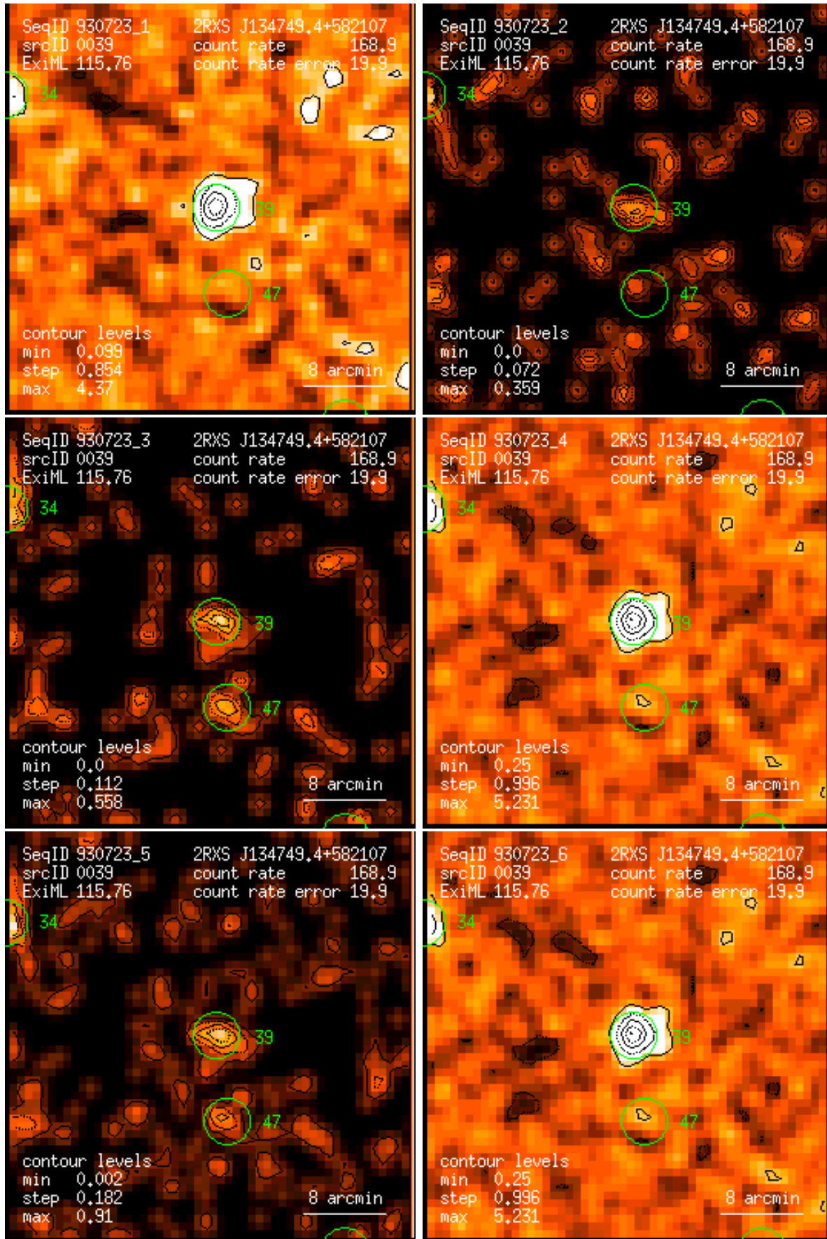
Figure 39: RASS 930723: detection 0039: band rate images, Gaussian filter: (1) PSPC channels 11 – 41, (2) 52 – 90, (3) 91 – 201, (4) 11 – 235, (5) 52 – 201, (6) 11 – 201. Broad band rates in counts/ks. Band rate contour levels in counts/ks/arcmin 2 .
