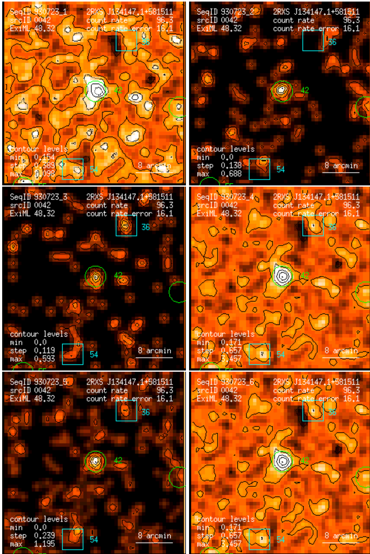
Figure 42: RASS 930723: detection 0042: band rate images, Gaussian filter: (1) PSPC channels 11 – 41, (2) 52 – 90, (3) 91 – 201, (4) 11 – 235, (5) 52 – 201, (6) 11 – 201. Broad band rates in counts/ks. Band rate contour levels in counts/ks/arcmin 2 .
