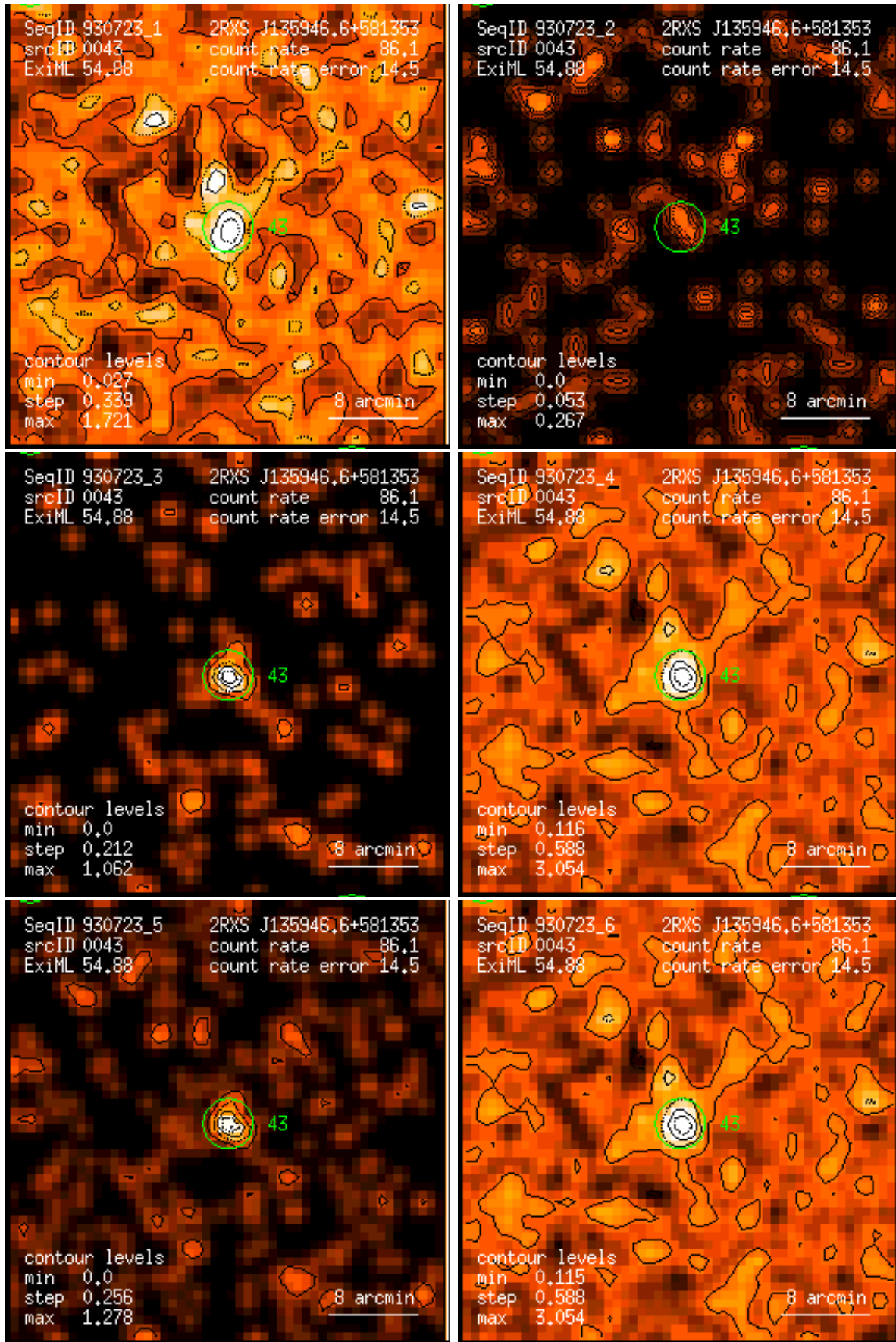
Figure 43: RASS 930723: detection 0043: band rate images, Gaussian filter: (1) PSPC channels 11 – 41, (2) 52 – 90, (3) 91 – 201, (4) 11 – 235, (5) 52 – 201, (6) 11 – 201. Broad band rates in counts/ks. Band rate contour levels in counts/ks/arcmin 2 .
