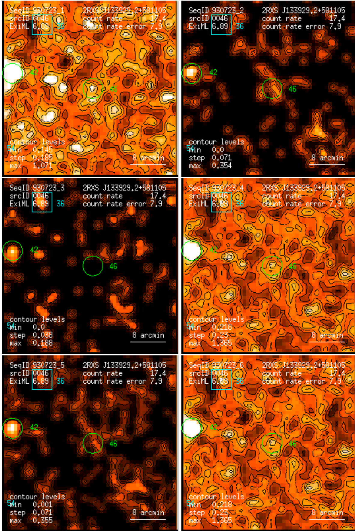
Figure 46: RASS 930723: detection 0046: band rate images, Gaussian filter: (1) PSPC channels 11 – 41, (2) 52 – 90, (3) 91 – 201, (4) 11 – 235, (5) 52 – 201, (6) 11 – 201. Broad band rates in counts/ks. Band rate contour levels in counts/ks/arcmin 2 .
