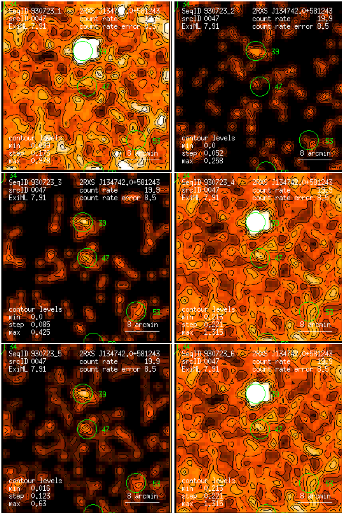
Figure 47: RASS 930723: detection 0047: band rate images, Gaussian filter: (1) PSPC channels 11 – 41, (2) 52 – 90, (3) 91 – 201, (4) 11 – 235, (5) 52 – 201, (6) 11 – 201. Broad band rates in counts/ks. Band rate contour levels in counts/ks/arcmin 2 .
