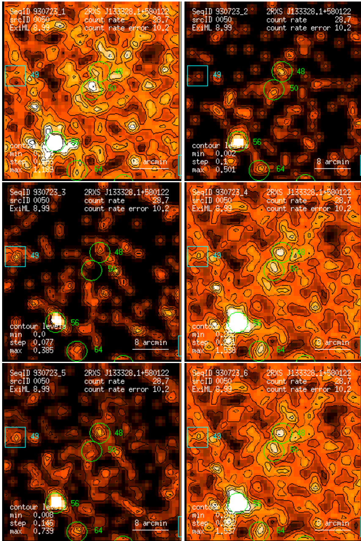
Figure 50: RASS 930723: detection 0050: band rate images, Gaussian filter: (1) PSPC channels 11 – 41, (2) 52 – 90, (3) 91 – 201, (4) 11 – 235, (5) 52 – 201, (6) 11 – 201. Broad band rates in counts/ks. Band rate contour levels in counts/ks/arcmin 2 .
