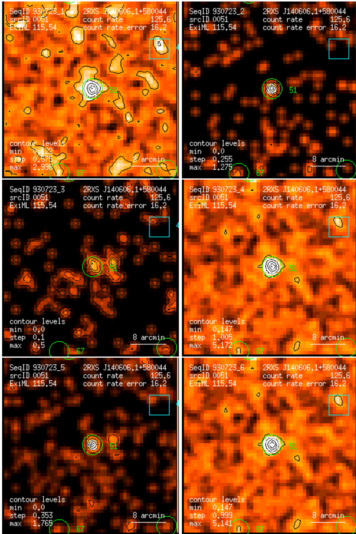
Figure 51: RASS 930723: detection 0051: band rate images, Gaussian filter: (1) PSPC channels 11 – 41, (2) 52 – 90, (3) 91 – 201, (4) 11 – 235, (5) 52 – 201, (6) 11 – 201. Broad band rates in counts/ks. Band rate contour levels in counts/ks/arcmin 2 .
