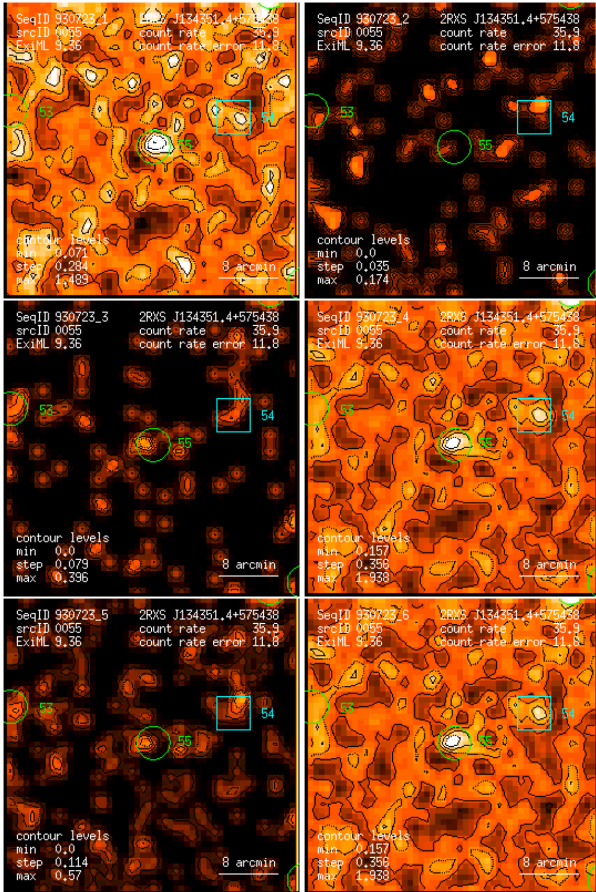
Figure 55: RASS 930723: detection 0055: band rate images, Gaussian filter: (1) PSPC channels 11 – 41, (2) 52 – 90, (3) 91 – 201, (4) 11 – 235, (5) 52 – 201, (6) 11 – 201. Broad band rates in counts/ks. Band rate contour levels in counts/ks/arcmin 2 .
