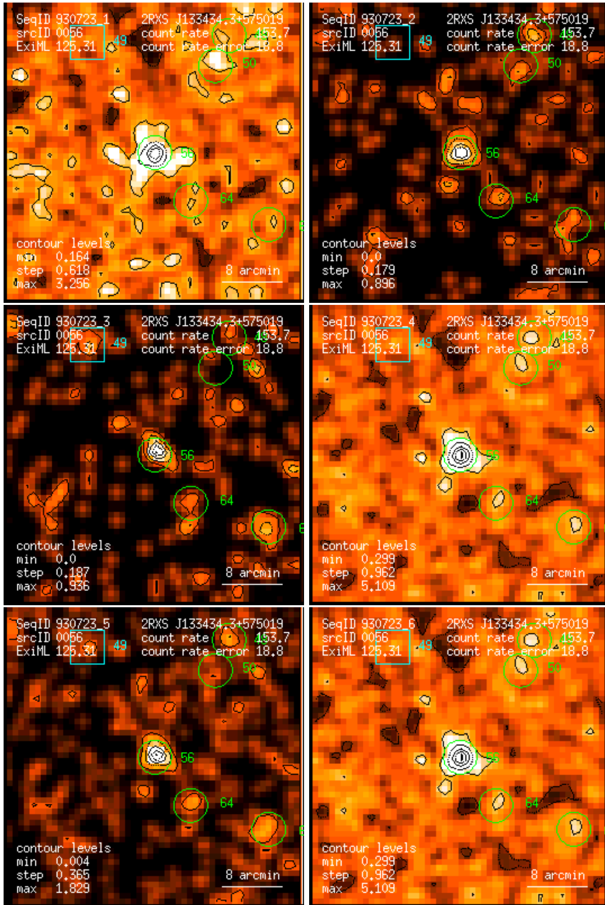
Figure 56: RASS 930723: detection 0056: band rate images, Gaussian filter: (1) PSPC channels 11 – 41, (2) 52 – 90, (3) 91 – 201, (4) 11 – 235, (5) 52 – 201, (6) 11 – 201. Broad band rates in counts/ks. Band rate contour levels in counts/ks/arcmin 2 .
