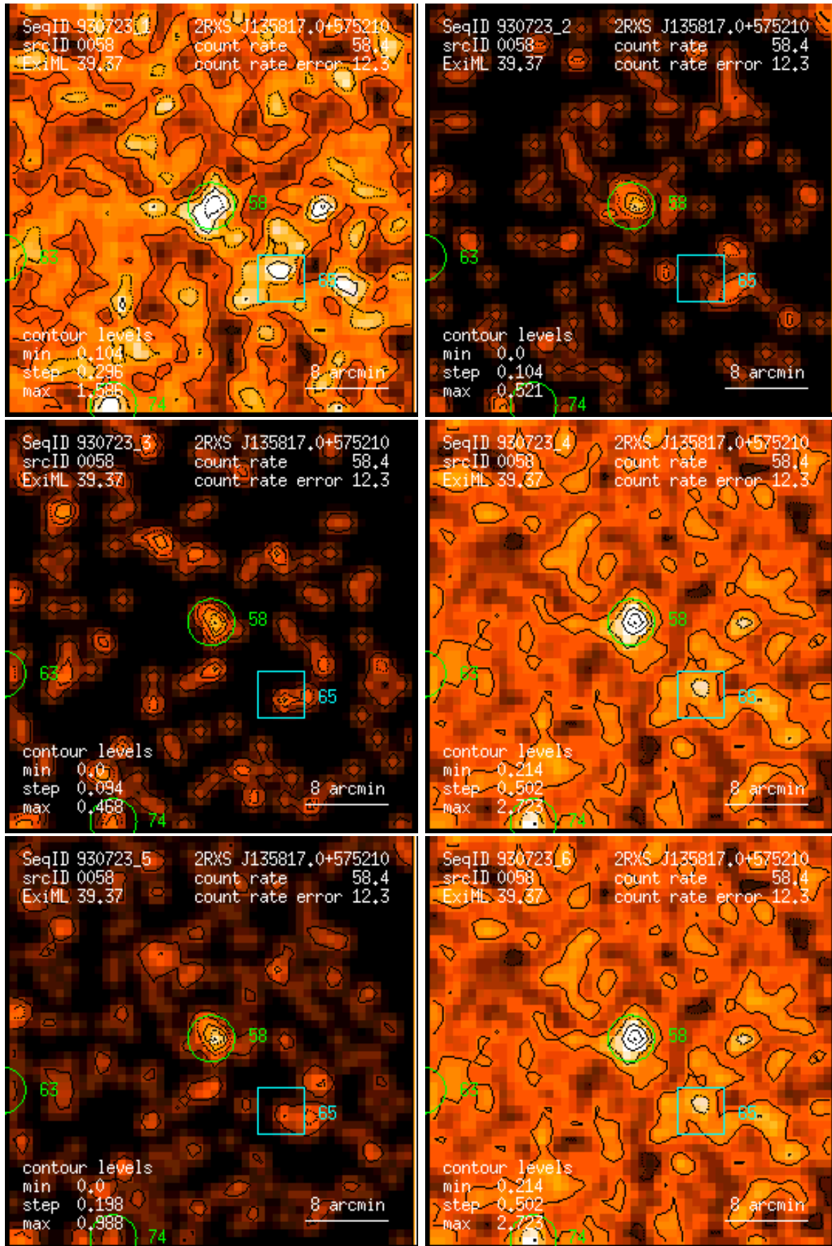
Figure 58: RASS 930723: detection 0058: band rate images, Gaussian filter: (1) PSPC channels 11 – 41, (2) 52 – 90, (3) 91 – 201, (4) 11 – 235, (5) 52 – 201, (6) 11 – 201. Broad band rates in counts/ks. Band rate contour levels in counts/ks/arcmin 2 .
