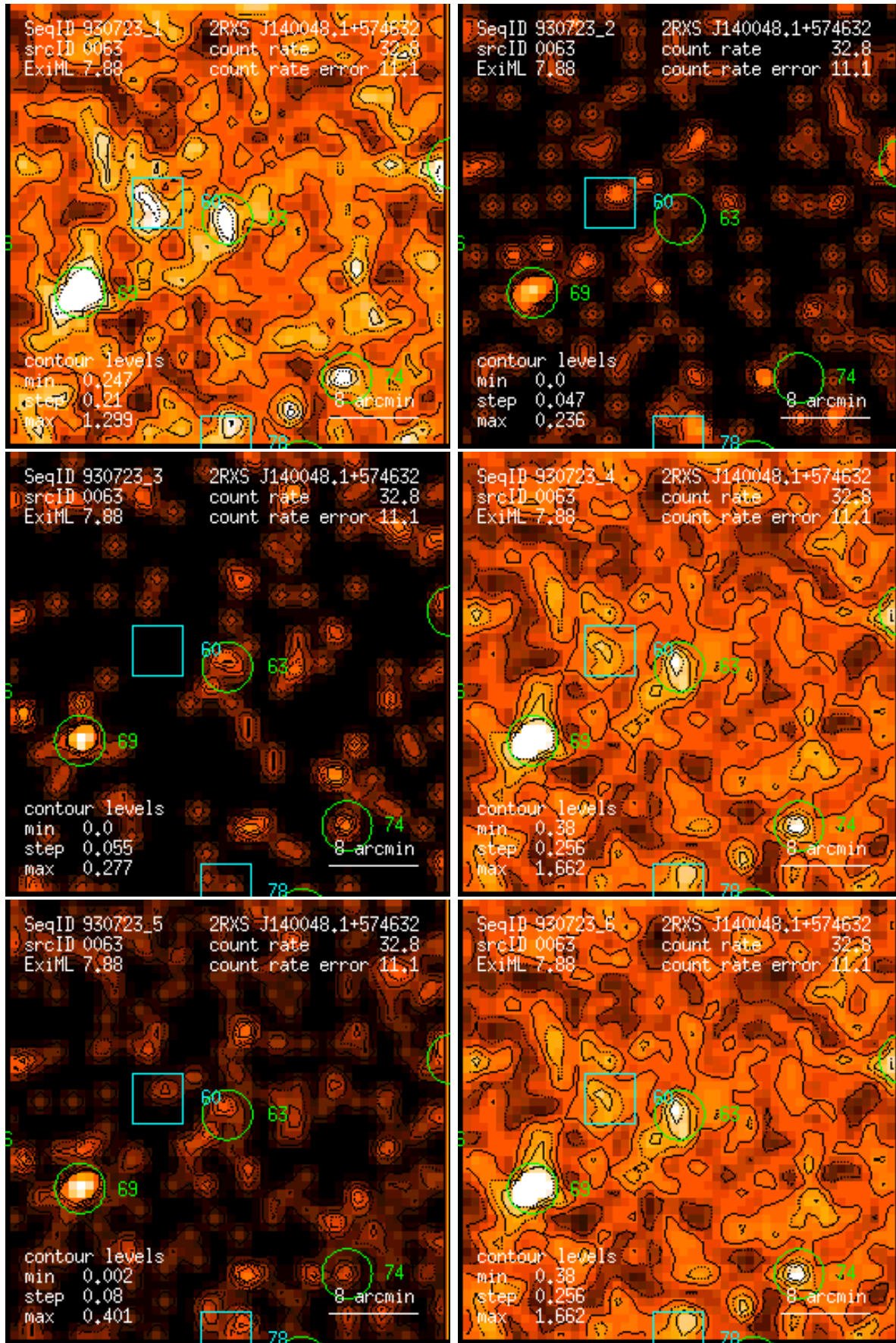
Figure 63: RASS 930723: detection 0063: band rate images, Gaussian filter: (1) PSPC channels 11 – 41, (2) 52 – 90, (3) 91 – 201, (4) 11 – 235, (5) 52 – 201, (6) 11 – 201. Broad band rates in counts/ks. Band rate contour levels in counts/ks/arcmin 2 .
