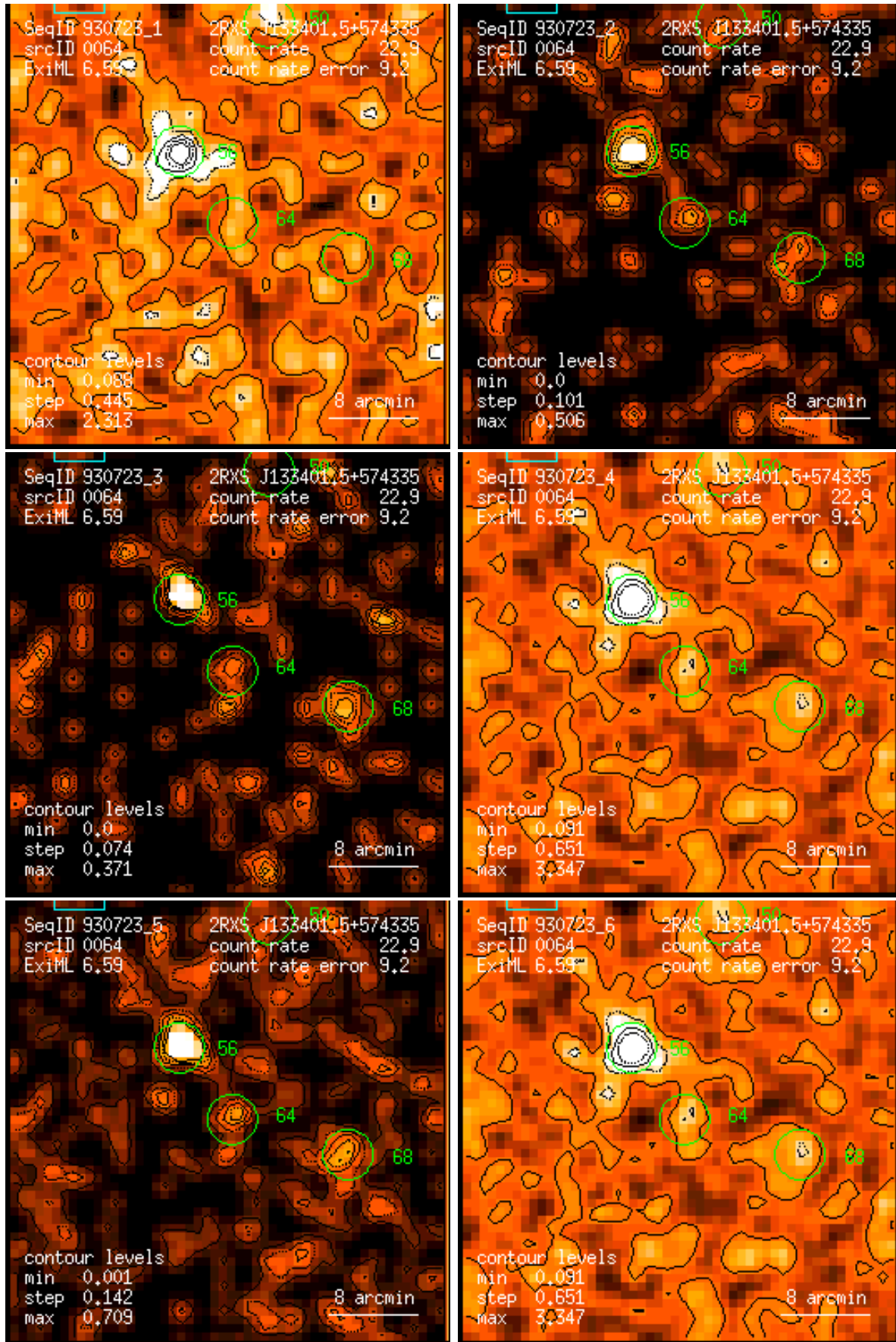
Figure 64: RASS 930723: detection 0064: band rate images, Gaussian filter: (1) PSPC channels 11 – 41, (2) 52 – 90, (3) 91 – 201, (4) 11 – 235, (5) 52 – 201, (6) 11 – 201. Broad band rates in counts/ks. Band rate contour levels in counts/ks/arcmin 2 .
