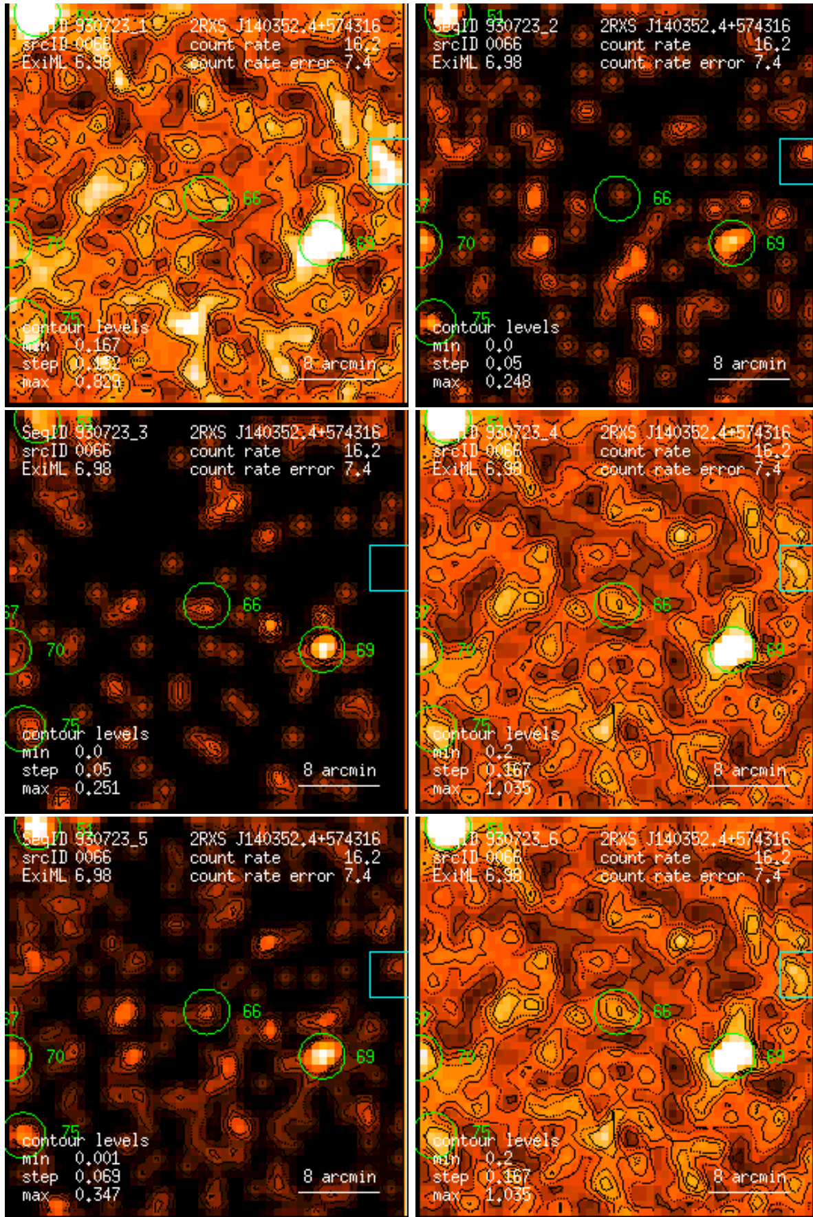
Figure 66: RASS 930723: detection 0066: band rate images, Gaussian filter: (1) PSPC channels 11 – 41, (2) 52 – 90, (3) 91 – 201, (4) 11 – 235, (5) 52 – 201, (6) 11 – 201. Broad band rates in counts/ks. Band rate contour levels in counts/ks/arcmin 2 .
