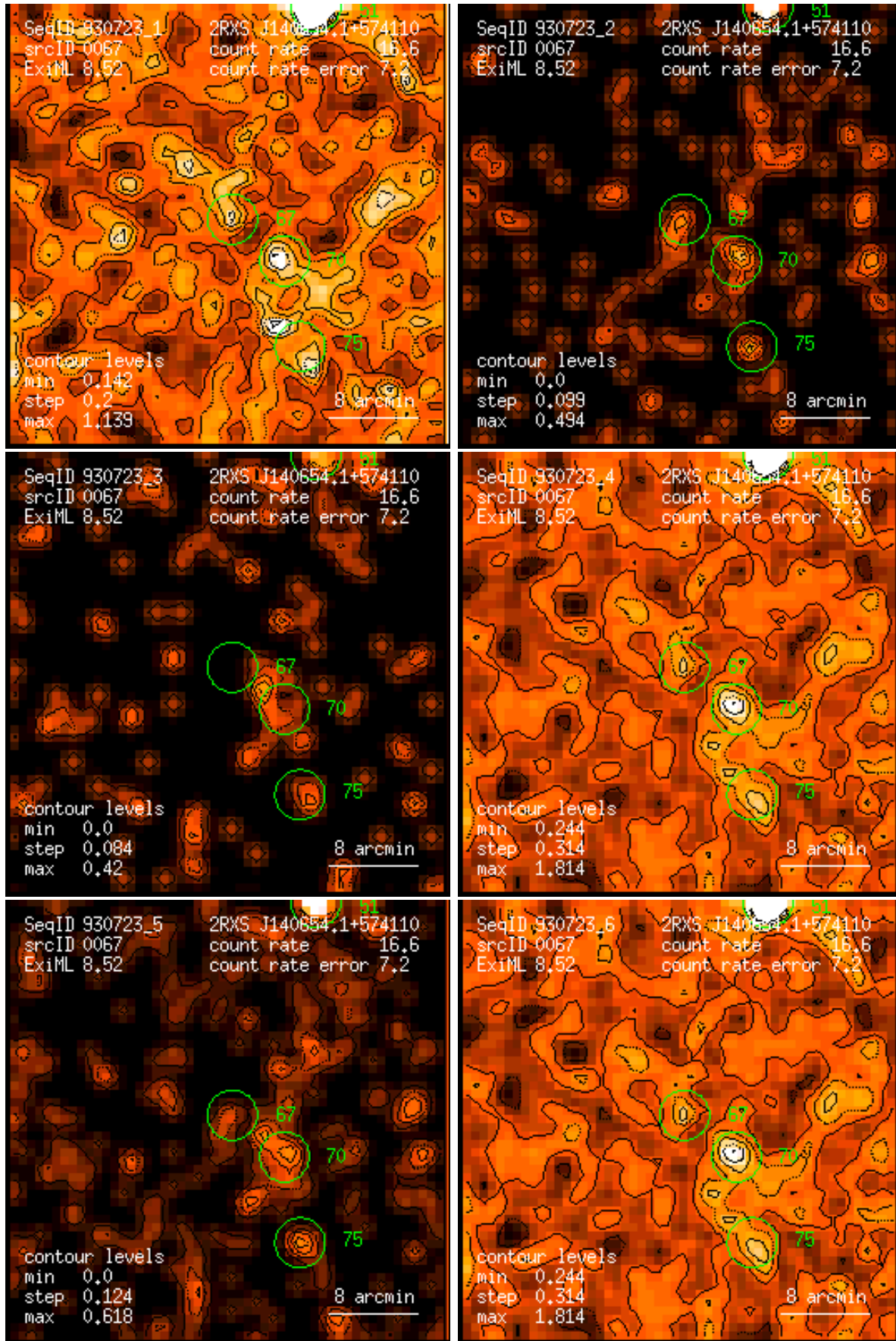
Figure 67: RASS 930723: detection 0067: band rate images, Gaussian filter: (1) PSPC channels 11 – 41, (2) 52 – 90, (3) 91 – 201, (4) 11 – 235, (5) 52 – 201, (6) 11 – 201. Broad band rates in counts/ks. Band rate contour levels in counts/ks/arcmin 2 .
