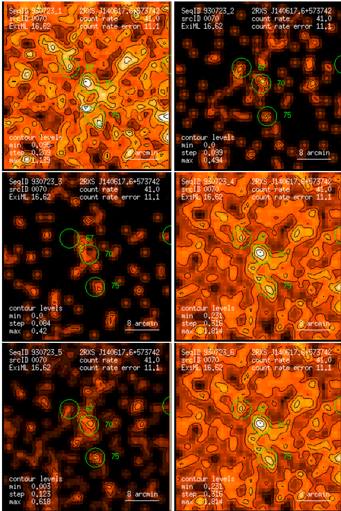
Figure 70: RASS 930723: detection 0070: band rate images, Gaussian filter: (1) PSPC channels 11 – 41, (2) 52 – 90, (3) 91 – 201, (4) 11 – 235, (5) 52 – 201, (6) 11 – 201. Broad band rates in counts/ks. Band rate contour levels in counts/ks/arcmin 2 .
