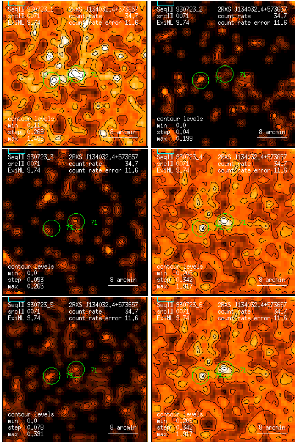
Figure 71: RASS 930723: detection 0071: band rate images, Gaussian filter: (1) PSPC channels 11 – 41, (2) 52 – 90, (3) 91 – 201, (4) 11 – 235, (5) 52 – 201, (6) 11 – 201. Broad band rates in counts/ks. Band rate contour levels in counts/ks/arcmin 2 .
