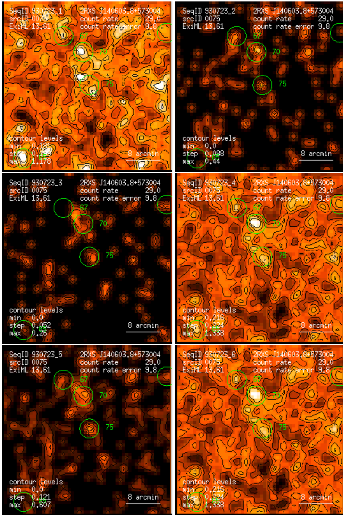
Figure 75: RASS 930723: detection 0075: band rate images, Gaussian filter: (1) PSPC channels 11 – 41, (2) 52 – 90, (3) 91 – 201, (4) 11 – 235, (5) 52 – 201, (6) 11 – 201. Broad band rates in counts/ks. Band rate contour levels in counts/ks/arcmin 2 .
