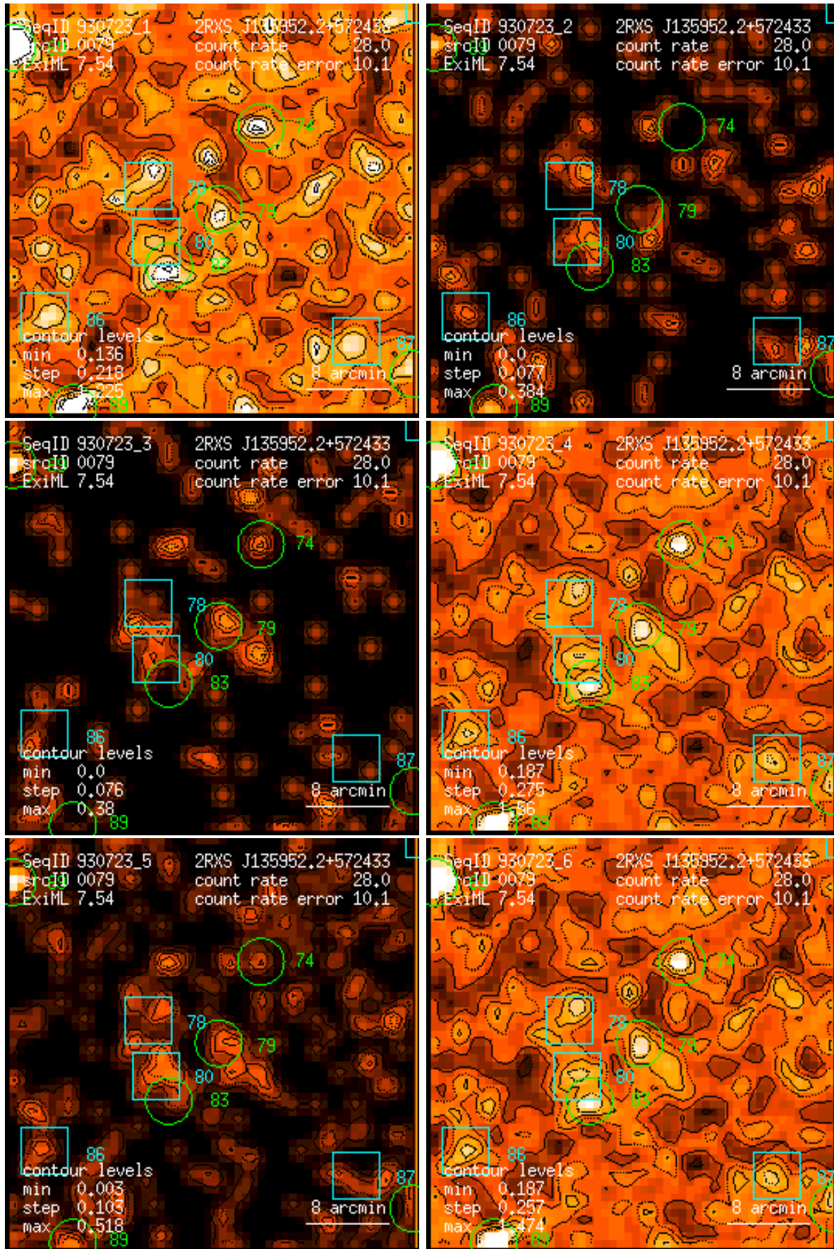
Figure 79: RASS 930723: detection 0079: band rate images, Gaussian filter: (1) PSPC channels 11 – 41, (2) 52 – 90, (3) 91 – 201, (4) 11 – 235, (5) 52 – 201, (6) 11 – 201. Broad band rates in counts/ks. Band rate contour levels in counts/ks/arcmin 2 .
