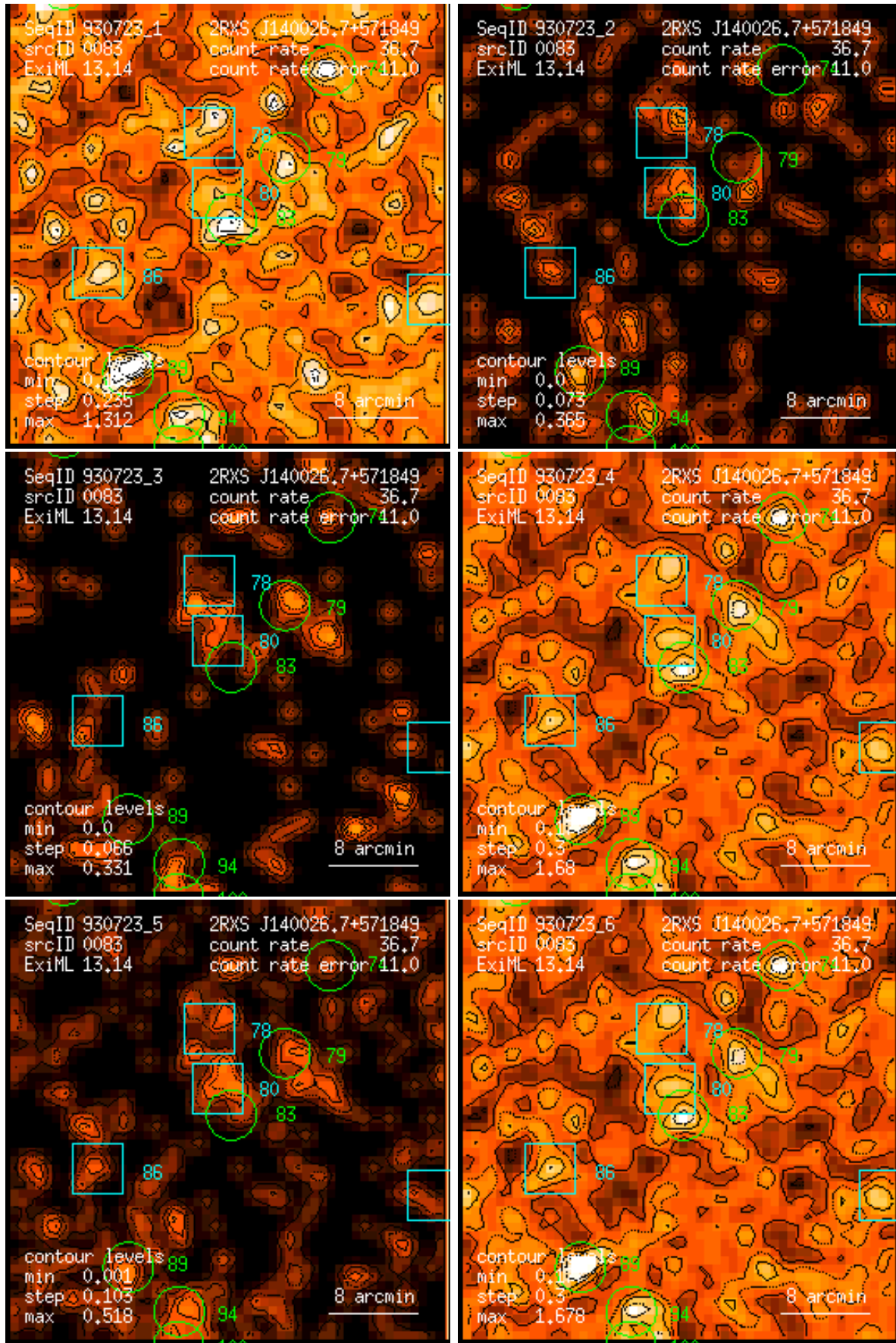
Figure 83: RASS 930723: detection 0083: band rate images, Gaussian filter: (1) PSPC channels 11 – 41, (2) 52 – 90, (3) 91 – 201, (4) 11 – 235, (5) 52 – 201, (6) 11 – 201. Broad band rates in counts/ks. Band rate contour levels in counts/ks/arcmin 2 .
