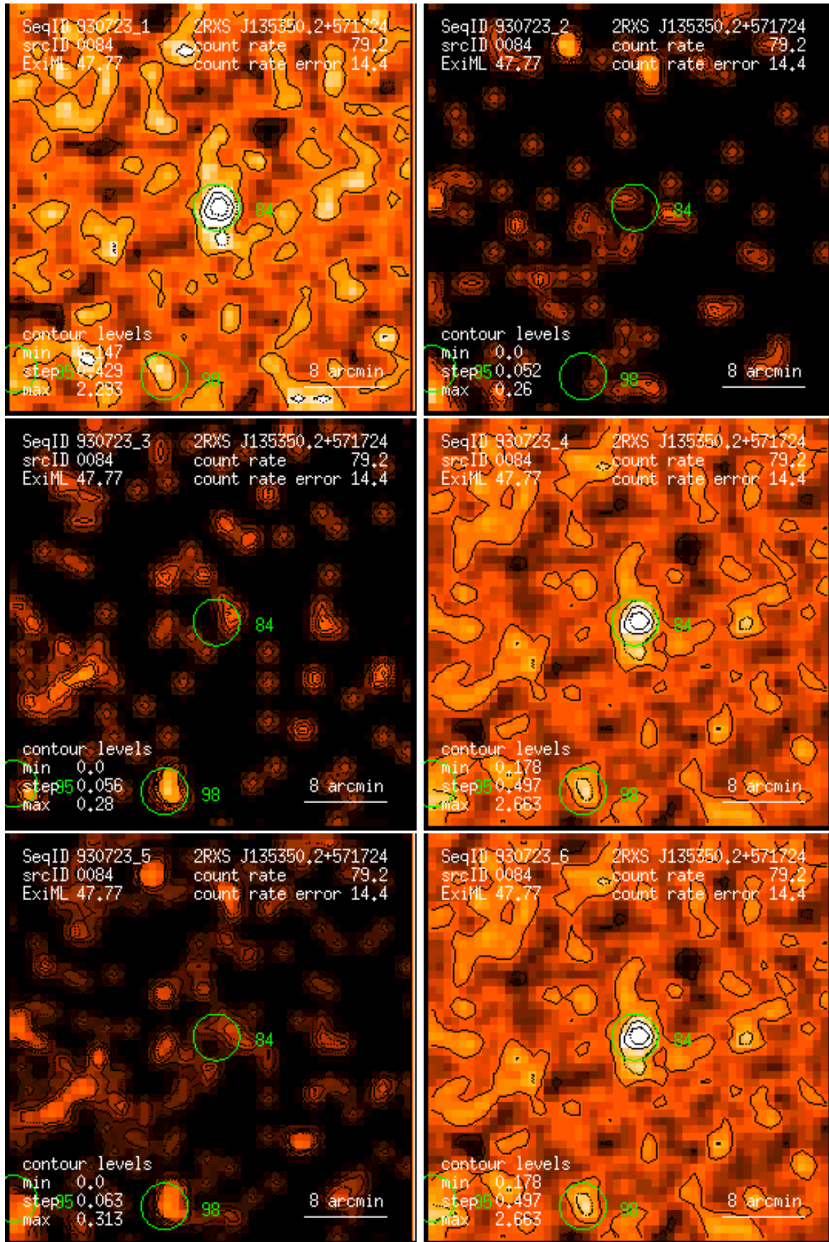
Figure 84: RASS 930723: detection 0084: band rate images, Gaussian filter: (1) PSPC channels 11 – 41, (2) 52 – 90, (3) 91 – 201, (4) 11 – 235, (5) 52 – 201, (6) 11 – 201. Broad band rates in counts/ks. Band rate contour levels in counts/ks/arcmin 2 .
