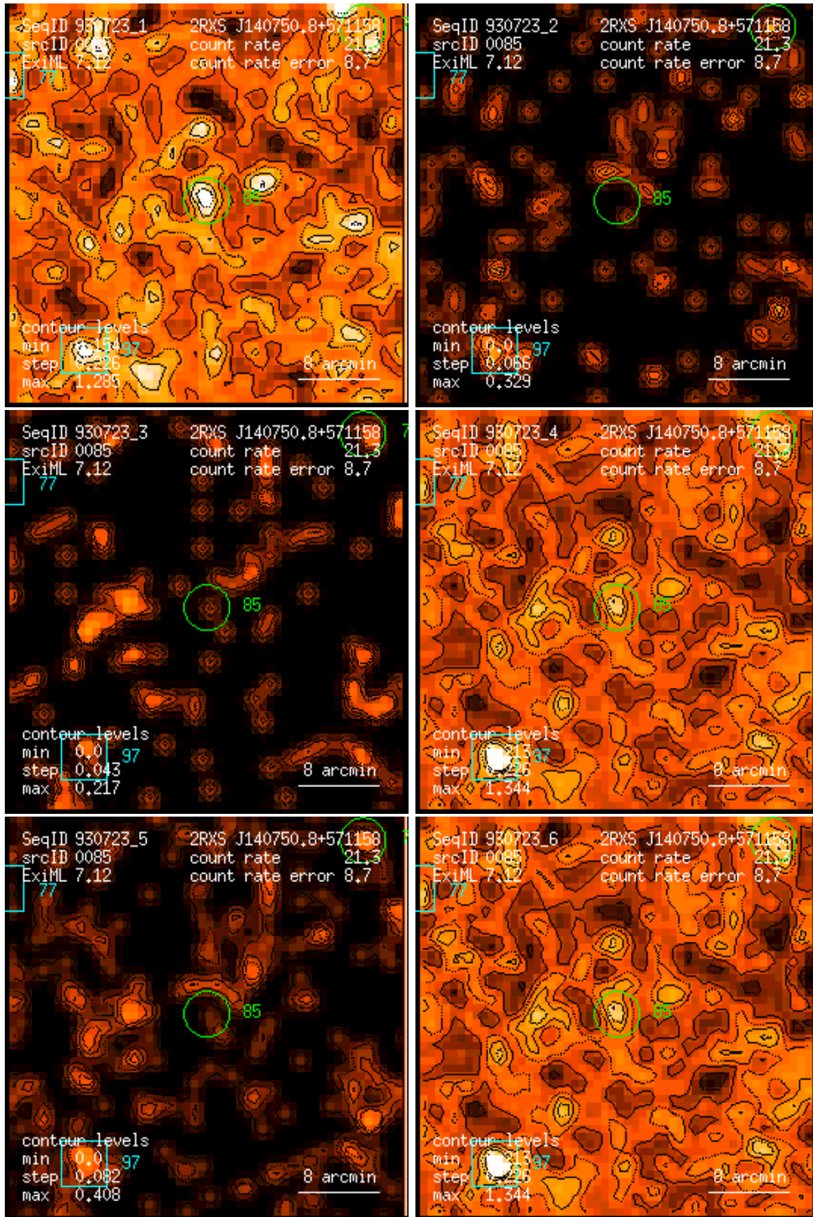
Figure 85: RASS 930723: detection 0085: band rate images, Gaussian filter: (1) PSPC channels 11 – 41, (2) 52 – 90, (3) 91 – 201, (4) 11 – 235, (5) 52 – 201, (6) 11 – 201. Broad band rates in counts/ks. Band rate contour levels in counts/ks/arcmin 2 .
