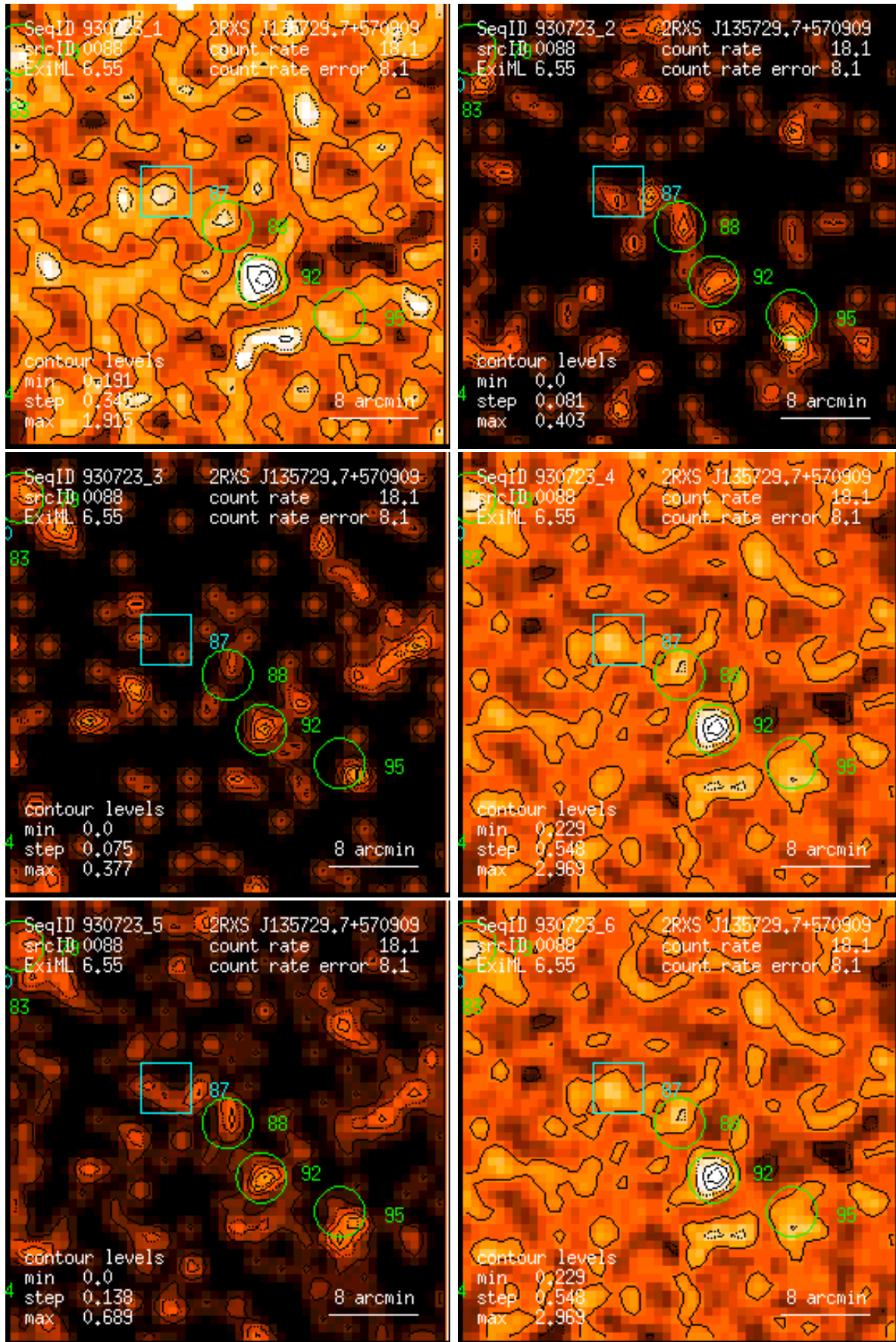
Figure 88: RASS 930723: detection 0088: band rate images, Gaussian filter: (1) PSPC channels 11 – 41, (2) 52 – 90, (3) 91 – 201, (4) 11 – 235, (5) 52 – 201, (6) 11 – 201. Broad band rates in counts/ks. Band rate contour levels in counts/ks/arcmin 2 .
