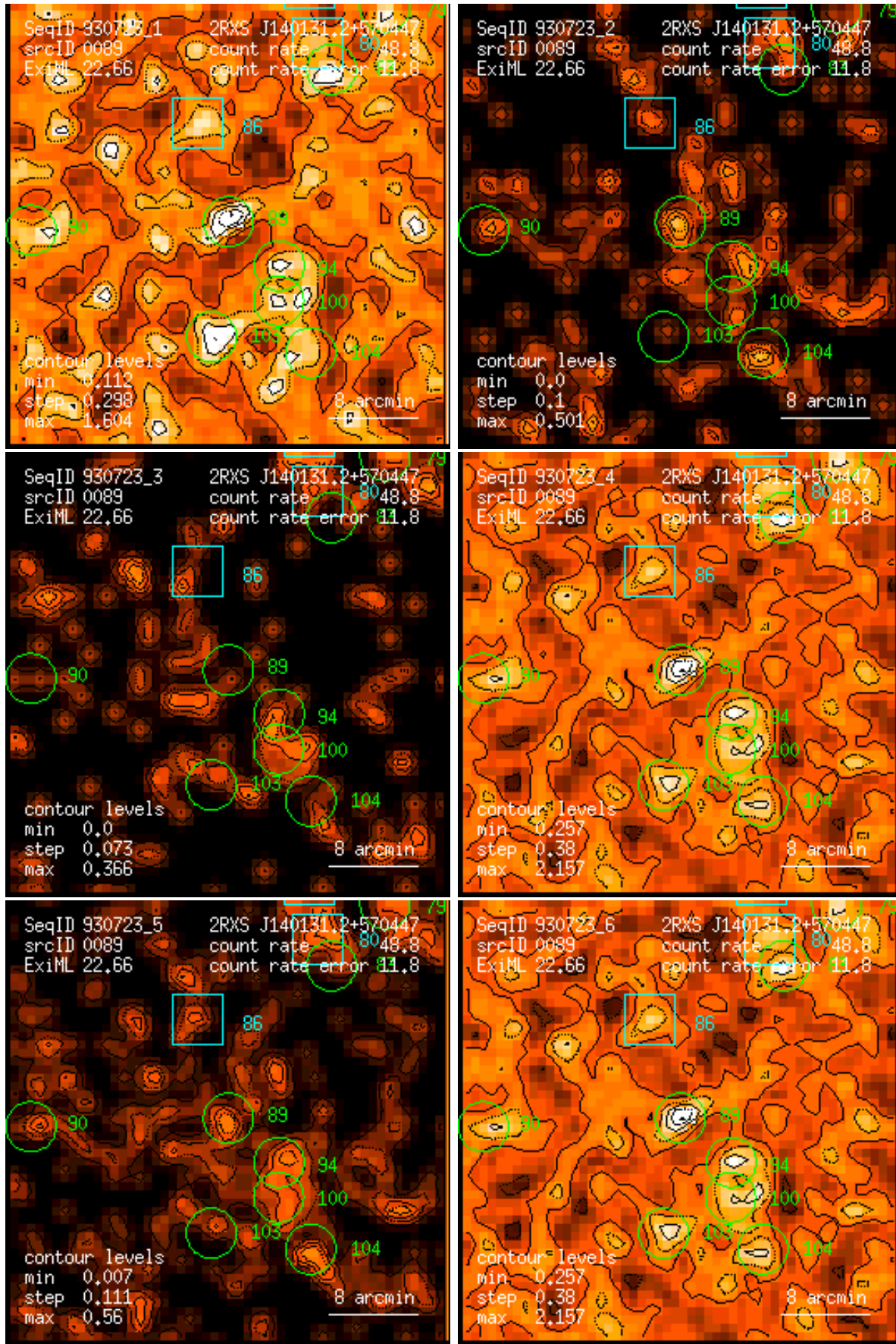
Figure 89: RASS 930723: detection 0089: band rate images, Gaussian filter: (1) PSPC channels 11 – 41, (2) 52 – 90, (3) 91 – 201, (4) 11 – 235, (5) 52 – 201, (6) 11 – 201. Broad band rates in counts/ks. Band rate contour levels in counts/ks/arcmin 2 .
