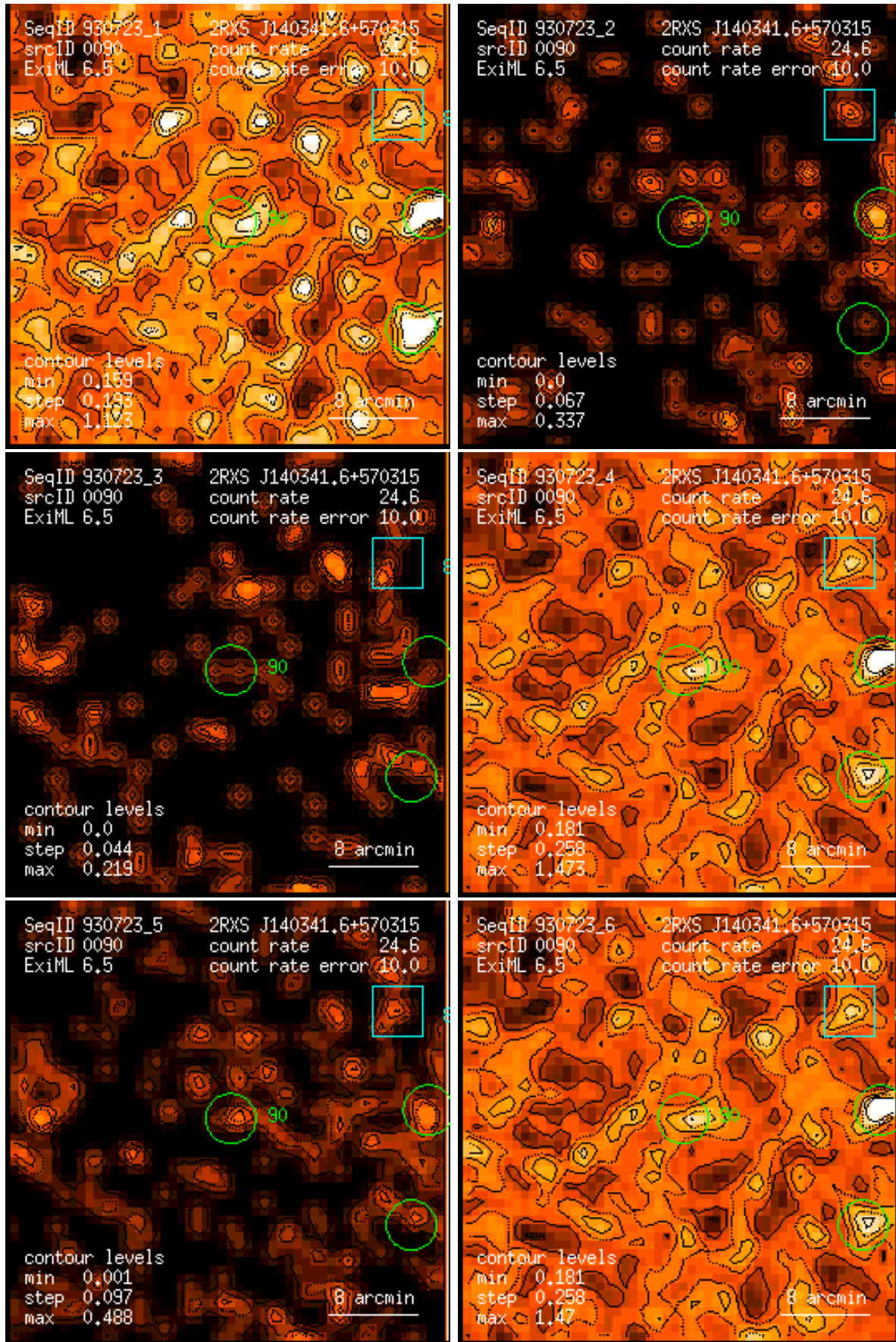
Figure 90: RASS 930723: detection 0090: band rate images, Gaussian filter: (1) PSPC channels 11 – 41, (2) 52 – 90, (3) 91 – 201, (4) 11 – 235, (5) 52 – 201, (6) 11 – 201. Broad band rates in counts/ks. Band rate contour levels in counts/ks/arcmin 2 .
