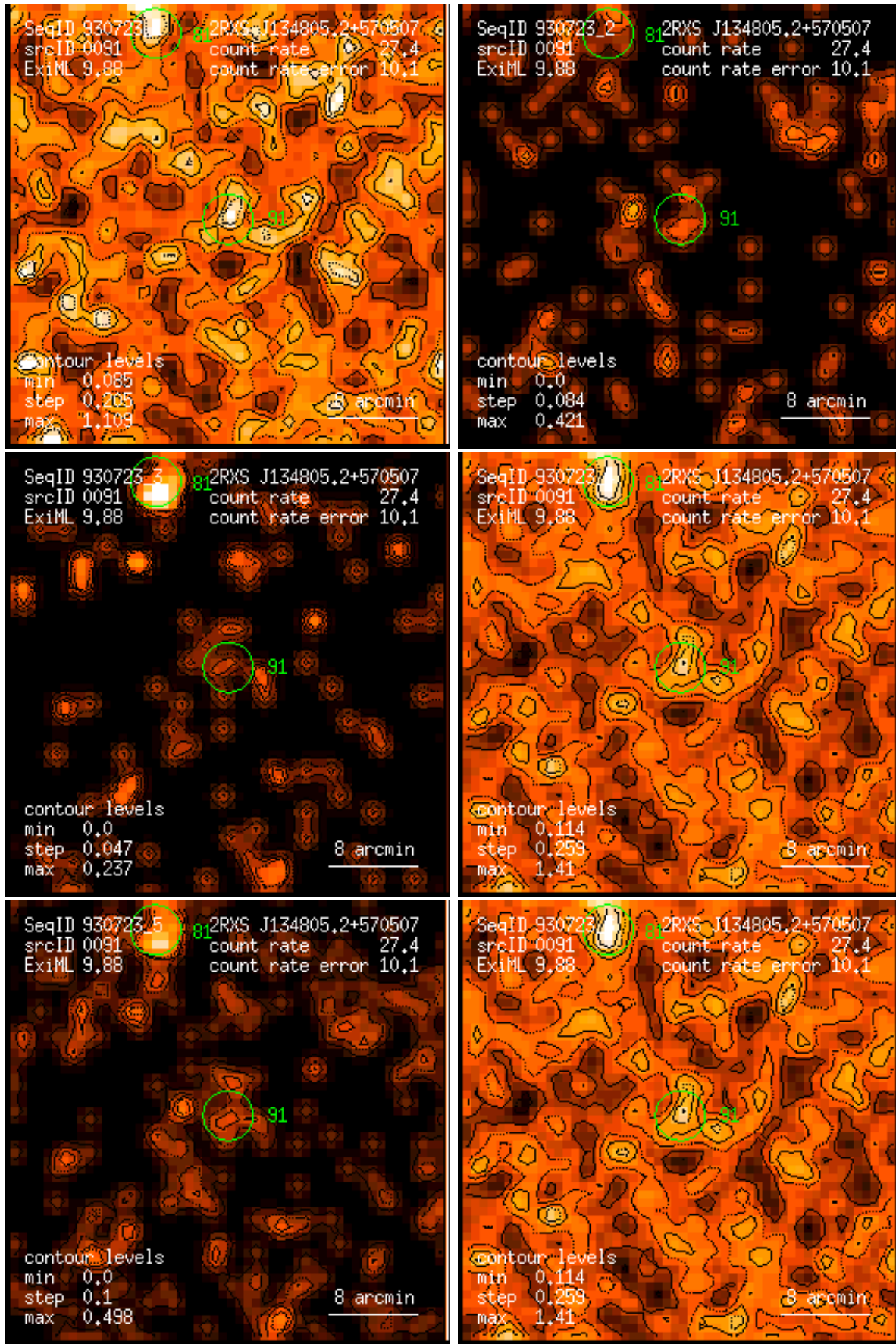
Figure 91: RASS 930723: detection 0091: band rate images, Gaussian filter: (1) PSPC channels 11 – 41, (2) 52 – 90, (3) 91 – 201, (4) 11 – 235, (5) 52 – 201, (6) 11 – 201. Broad band rates in counts/ks. Band rate contour levels in counts/ks/arcmin 2 .
