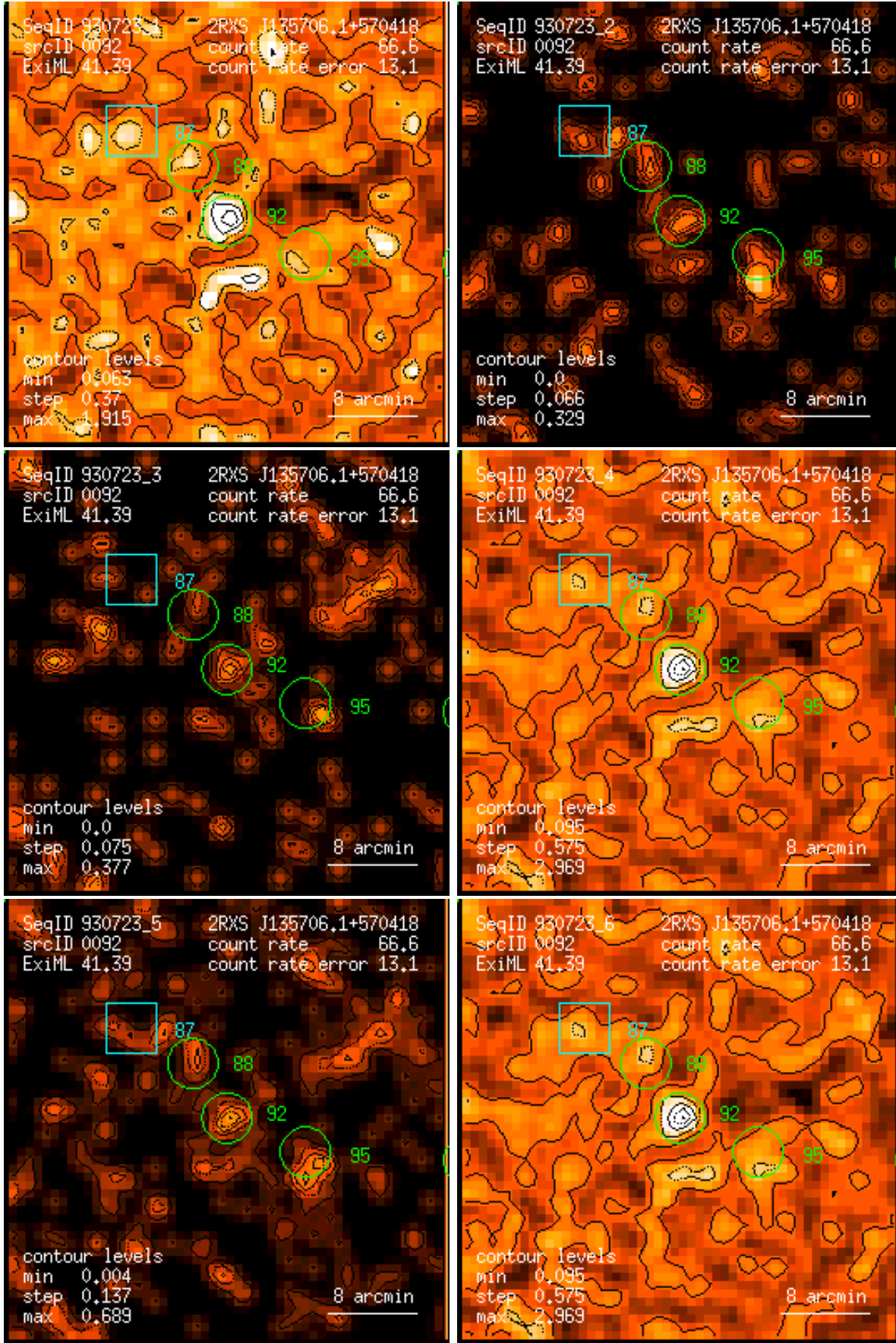
Figure 92: RASS 930723: detection 0092: band rate images, Gaussian filter: (1) PSPC channels 11 – 41, (2) 52 – 90, (3) 91 – 201, (4) 11 – 235, (5) 52 – 201, (6) 11 – 201. Broad band rates in counts/ks. Band rate contour levels in counts/ks/arcmin 2 .
