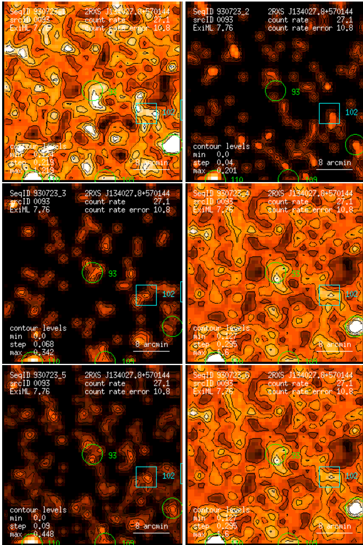
Figure 93: RASS 930723: detection 0093: band rate images, Gaussian filter: (1) PSPC channels 11 – 41, (2) 52 – 90, (3) 91 – 201, (4) 11 – 235, (5) 52 – 201, (6) 11 – 201. Broad band rates in counts/ks. Band rate contour levels in counts/ks/arcmin 2 .
