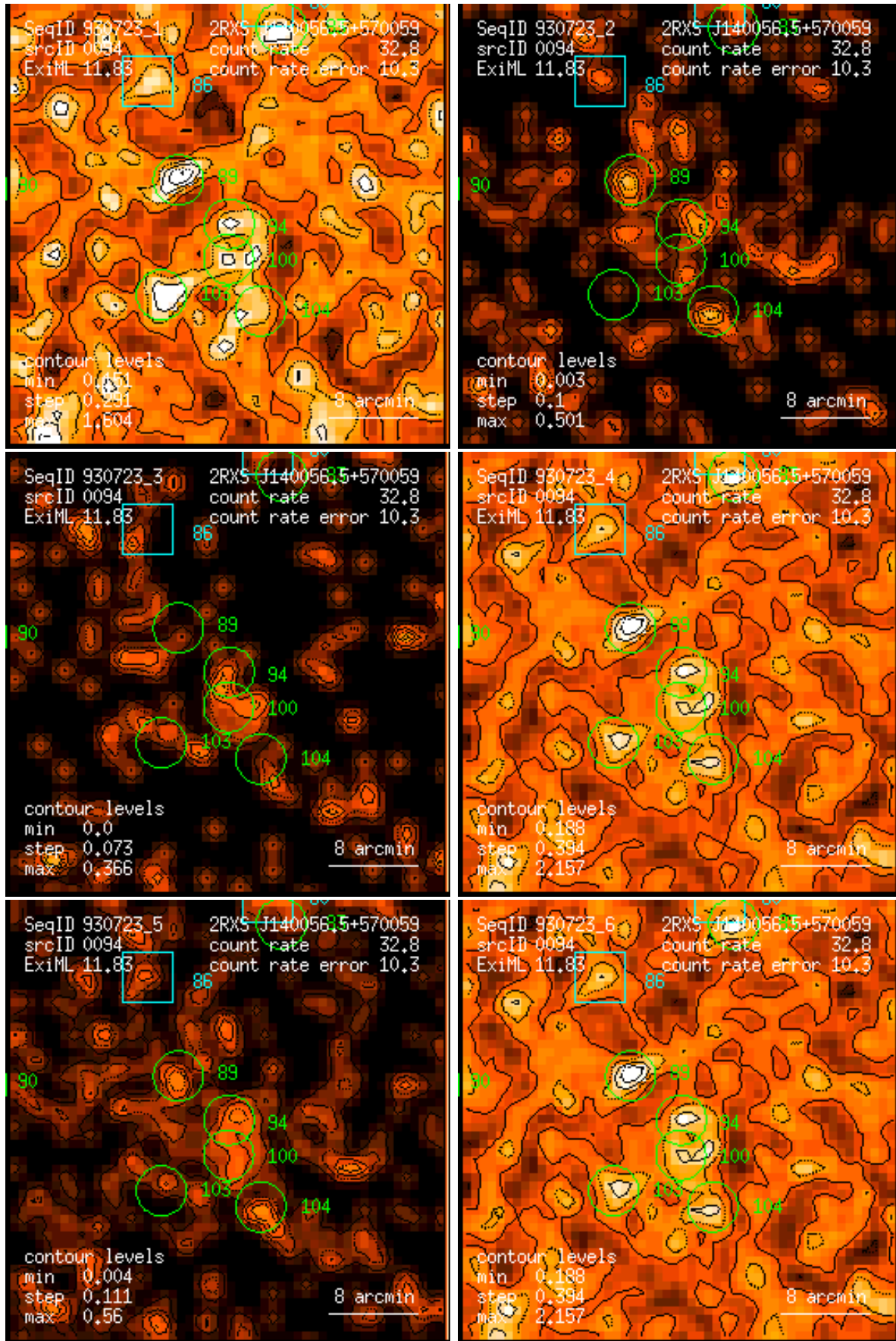
Figure 94: RASS 930723: detection 0094: band rate images, Gaussian filter: (1) PSPC channels 11 – 41, (2) 52 – 90, (3) 91 – 201, (4) 11 – 235, (5) 52 – 201, (6) 11 – 201. Broad band rates in counts/ks. Band rate contour levels in counts/ks/arcmin 2 .
