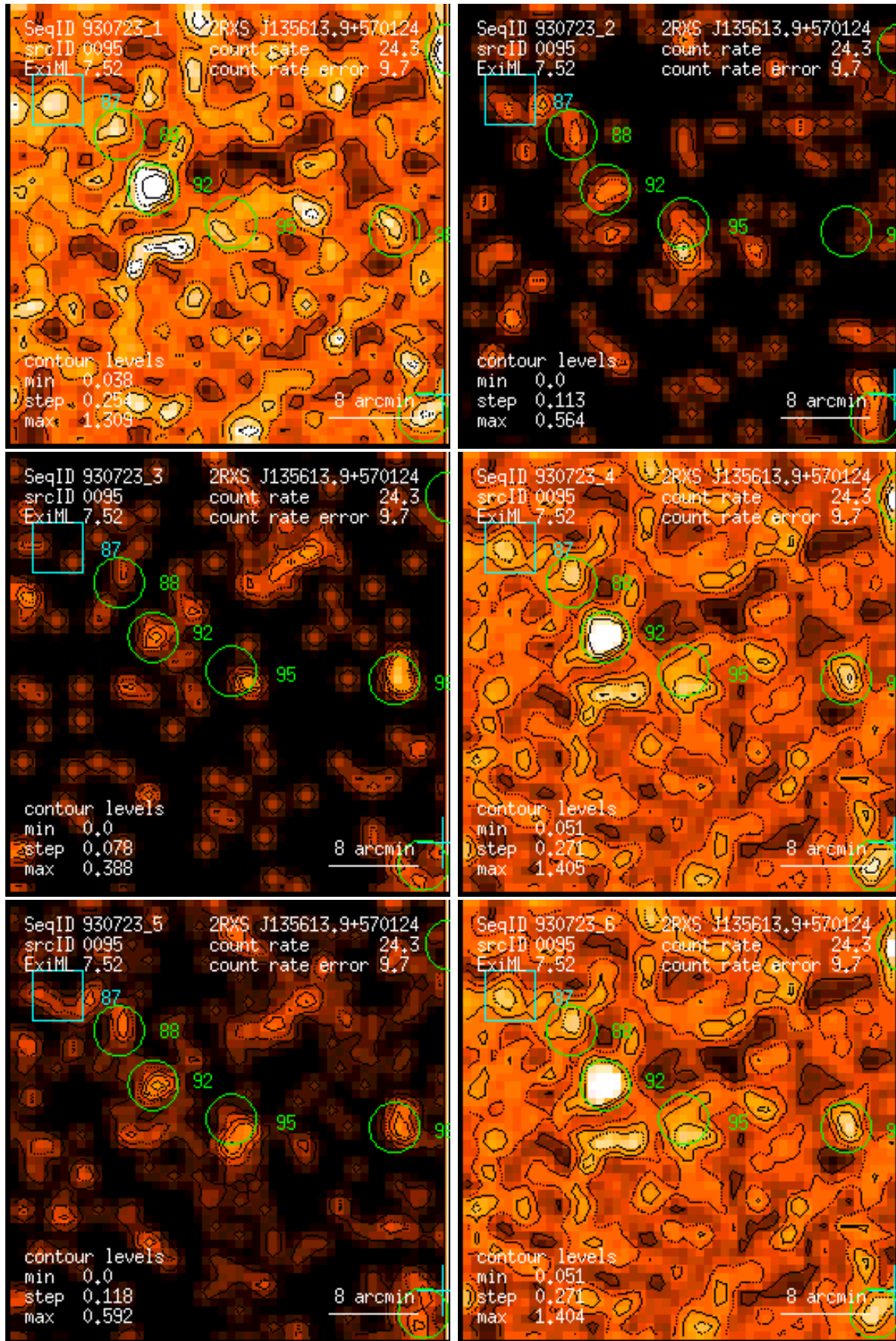
Figure 95: RASS 930723: detection 0095: band rate images, Gaussian filter: (1) PSPC channels 11 – 41, (2) 52 – 90, (3) 91 – 201, (4) 11 – 235, (5) 52 – 201, (6) 11 – 201. Broad band rates in counts/ks. Band rate contour levels in counts/ks/arcmin 2 .
