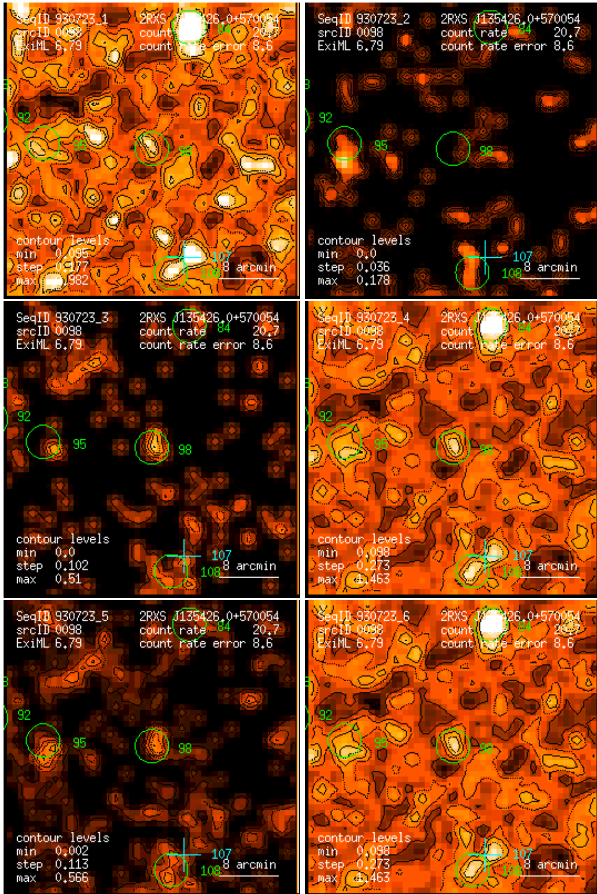
Figure 98: RASS 930723: detection 0098: band rate images, Gaussian filter: (1) PSPC channels 11 – 41, (2) 52 – 90, (3) 91 – 201, (4) 11 – 235, (5) 52 – 201, (6) 11 – 201. Broad band rates in counts/ks. Band rate contour levels in counts/ks/arcmin 2 .
