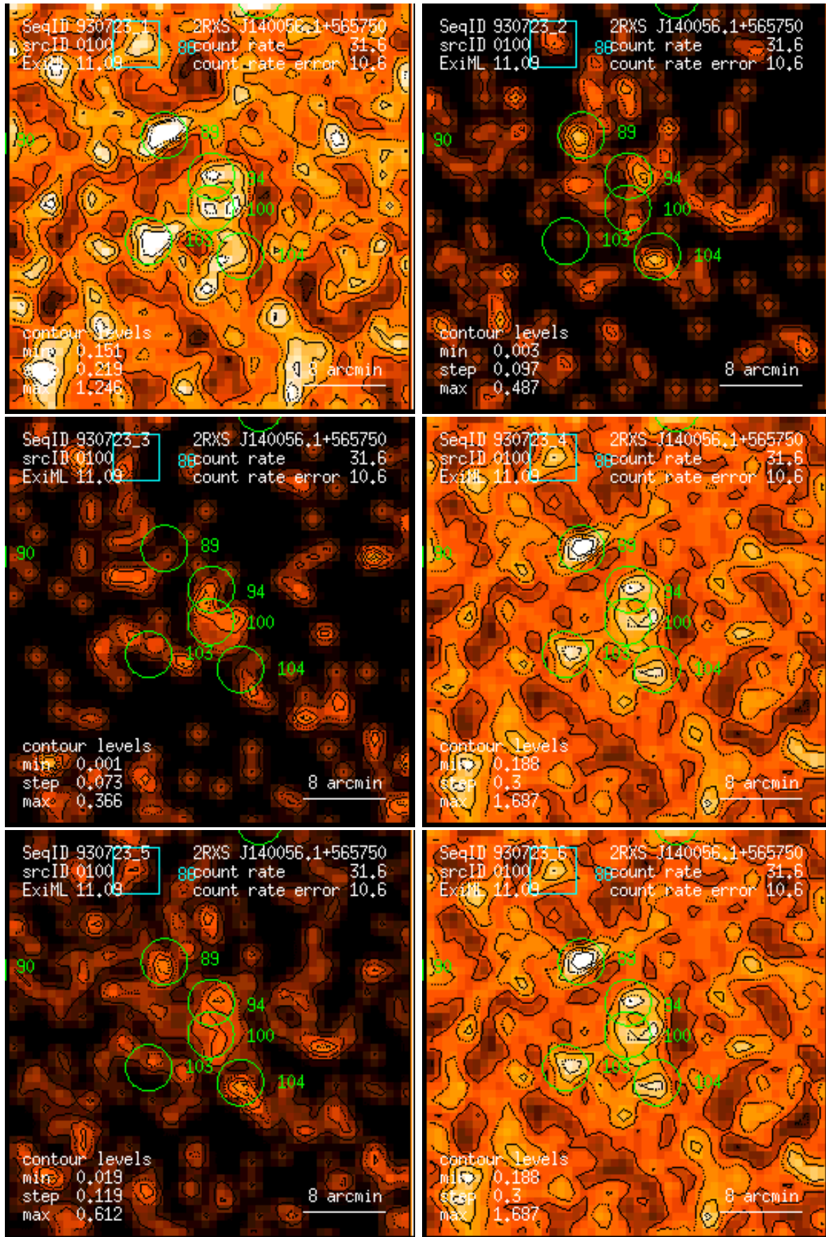
Figure 100: RASS 930723: detection 0100: band rate images, Gaussian filter: (1) PSPC channels 11 – 41, (2) 52 – 90, (3) 91 – 201, (4) 11 – 235, (5) 52 – 201, (6) 11 – 201. Broad band rates in counts/ks. Band rate contour levels in counts/ks/arcmin 2 .
