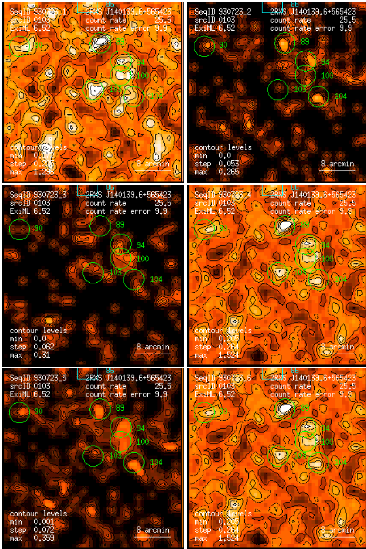
Figure 103: RASS 930723: detection 0103: band rate images, Gaussian filter: (1) PSPC channels 11 – 41, (2) 52 – 90, (3) 91 – 201, (4) 11 – 235, (5) 52 – 201, (6) 11 – 201. Broad band rates in counts/ks. Band rate contour levels in counts/ks/arcmin 2 .
