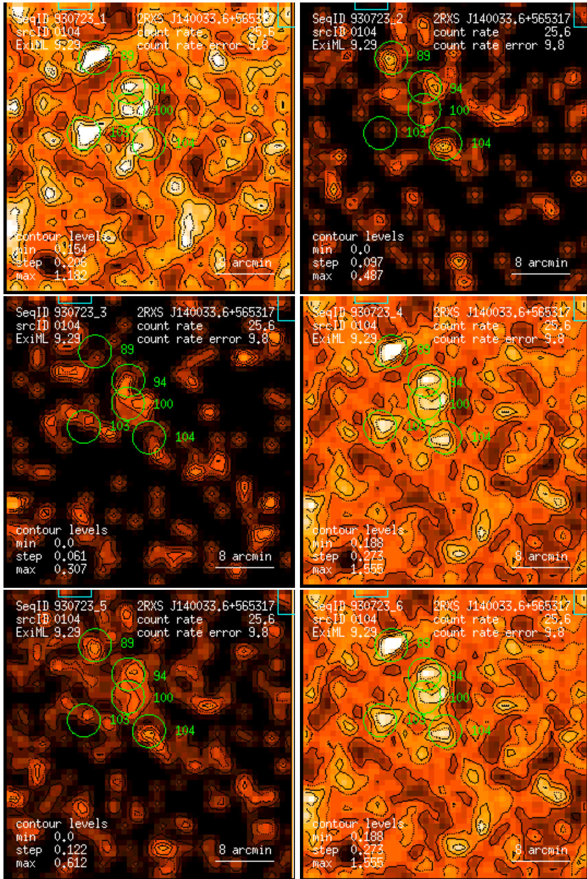
Figure 104: RASS 930723: detection 0104: band rate images, Gaussian filter: (1) PSPC channels 11 – 41, (2) 52 – 90, (3) 91 – 201, (4) 11 – 235, (5) 52 – 201, (6) 11 – 201. Broad band rates in counts/ks. Band rate contour levels in counts/ks/arcmin 2 .
